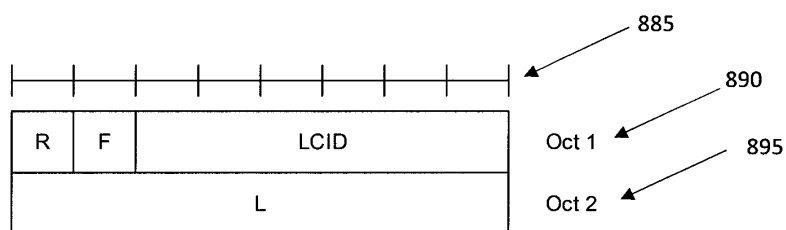
Figure 6.1.2-3: R/LCID MAC subheader
