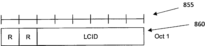
Figure 6.1.2-3: R/LCID MAC subheader
