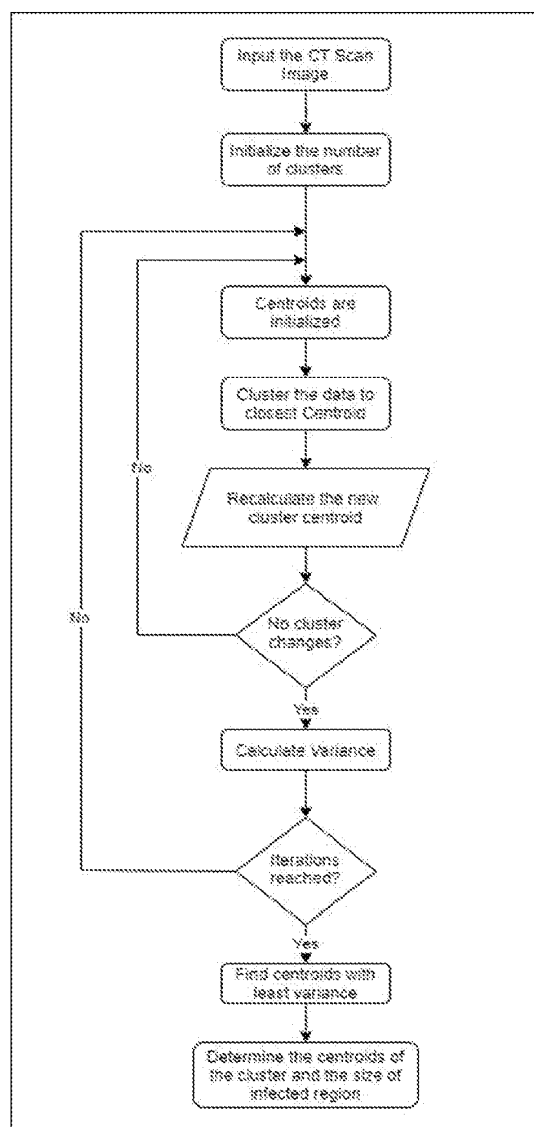
Figure 1. Flowchart for K-means clustering algorithm
