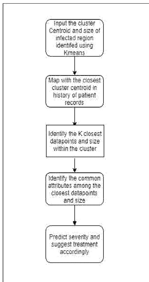
Figure 2. Flowchart for KNN classification algorithm
