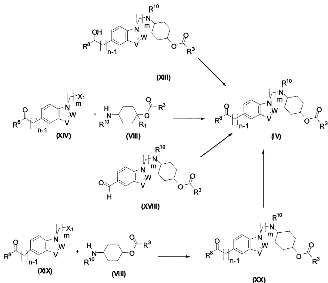
Scheme 3
