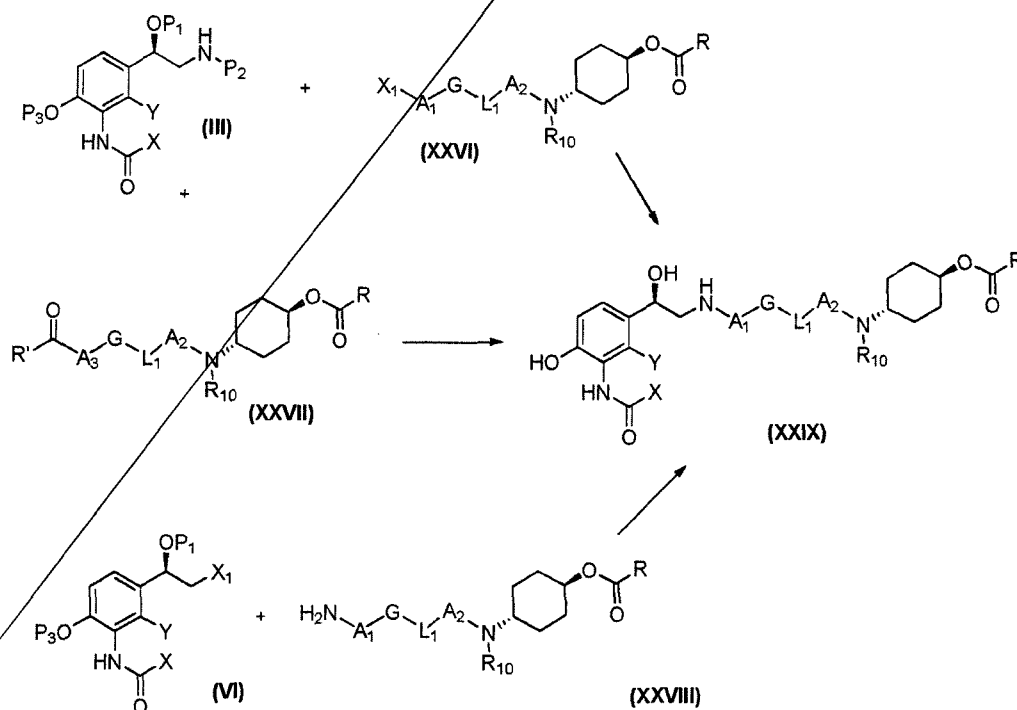
Scheme 6
