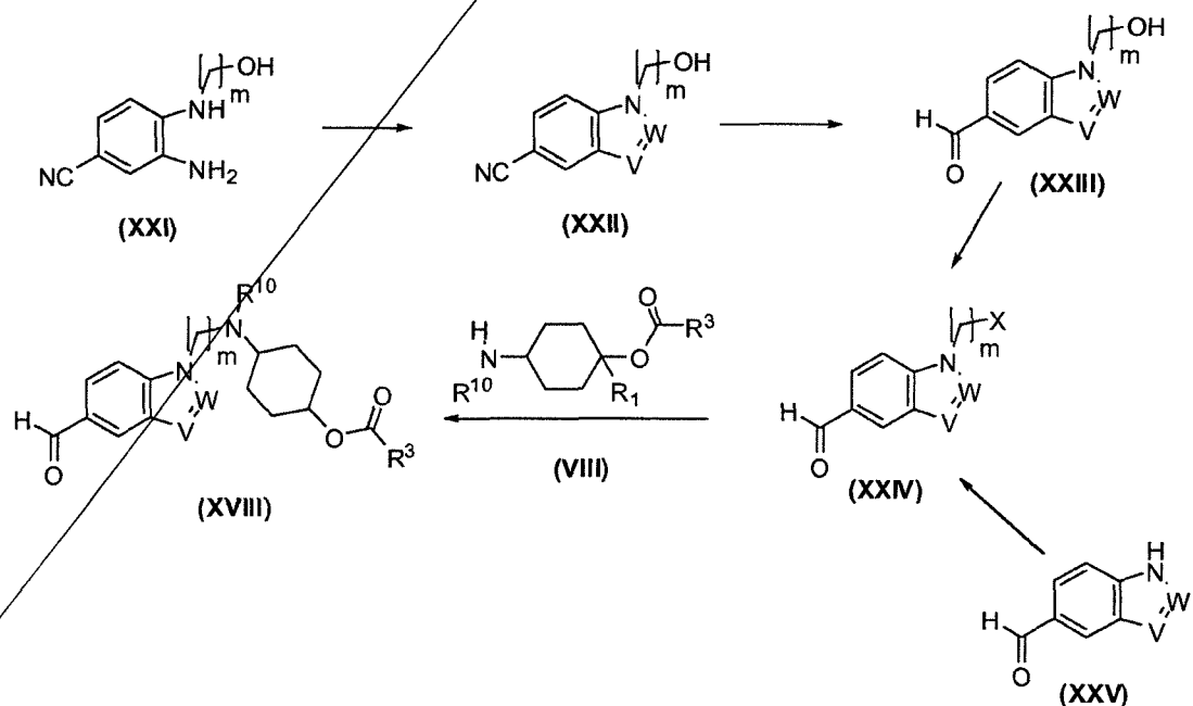
Scheme 5
