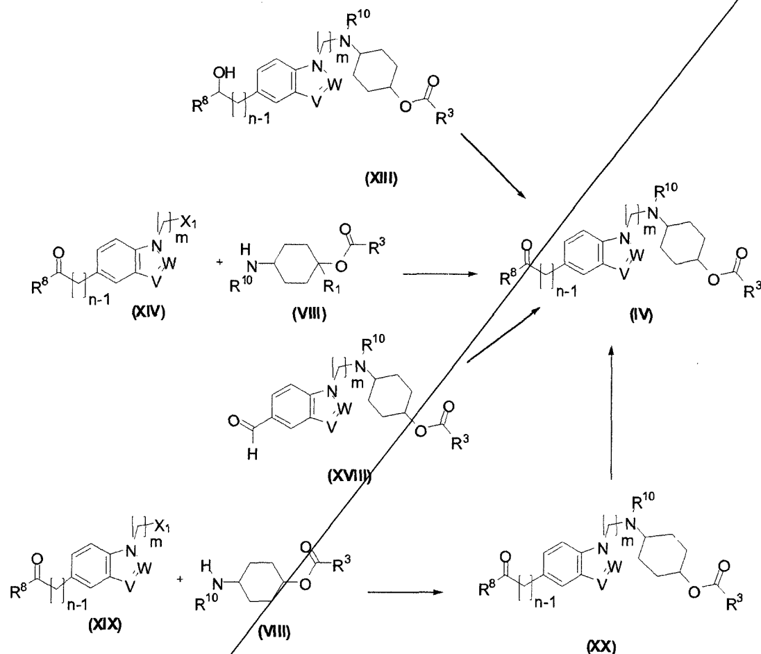
Scheme 3
