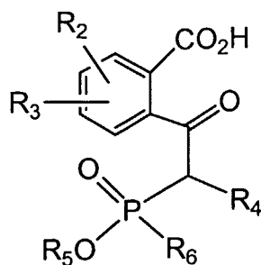
Formula (B').
