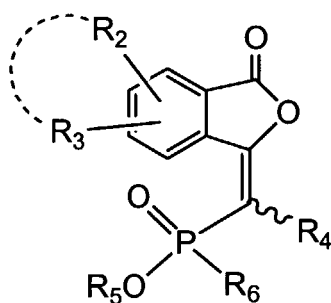
Formula (C)
