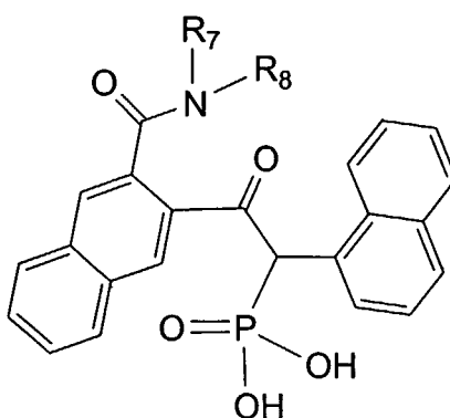
Formula (Ia)
