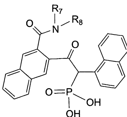
Formula (Ia)
