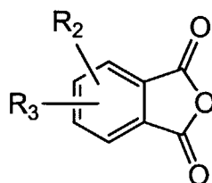
Formula (F)
