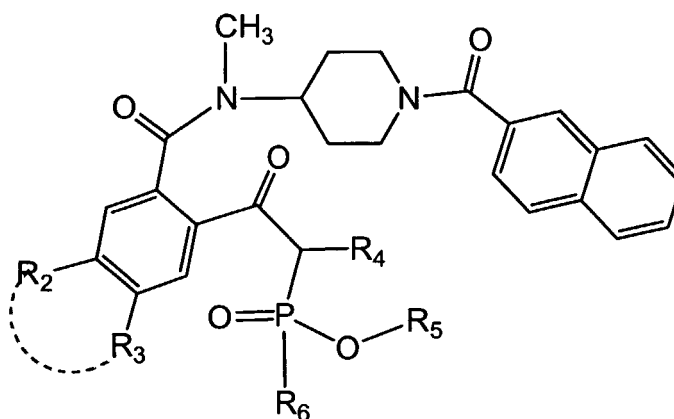
Formula (Ic)
