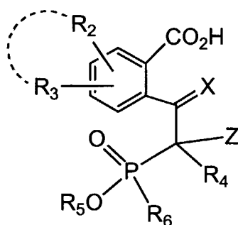
Formula (B)
