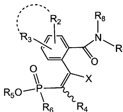
Formula (E)
