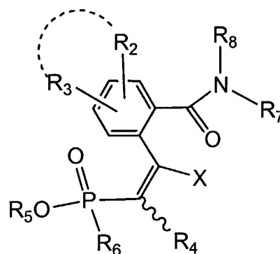
Formula (E)
