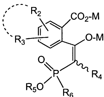
Formula (H)
