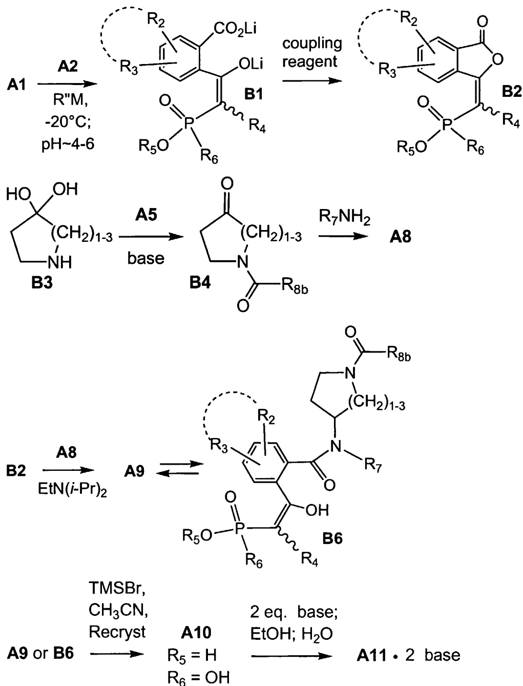
Scheme B
