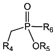
Formula (G)
