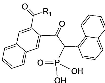
Formula (Ib)
