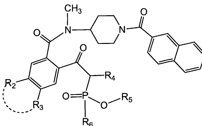
Formula (Ic)
