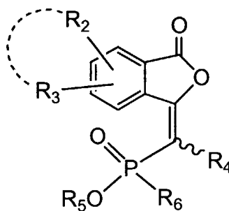
Formula (C)
