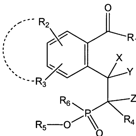
Formula (I)
