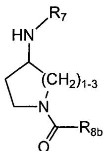
Formula (A')
