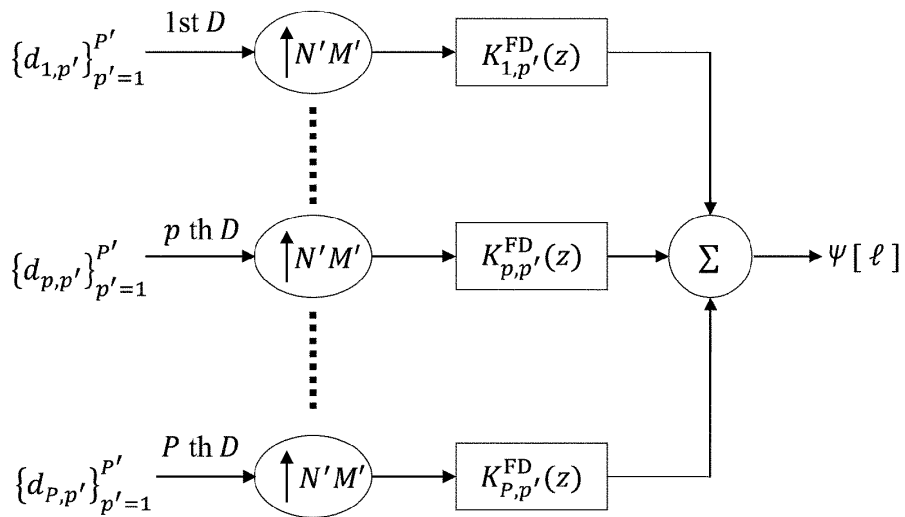
SFB for data embedded transmit FD signal
