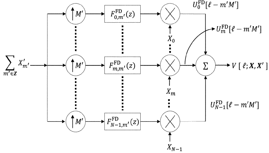
SFB for signature V[\ell; \mathbf{X}, \mathbf{X}']
