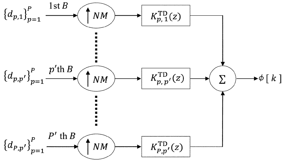
SFB for data embedded transmit TD signal
