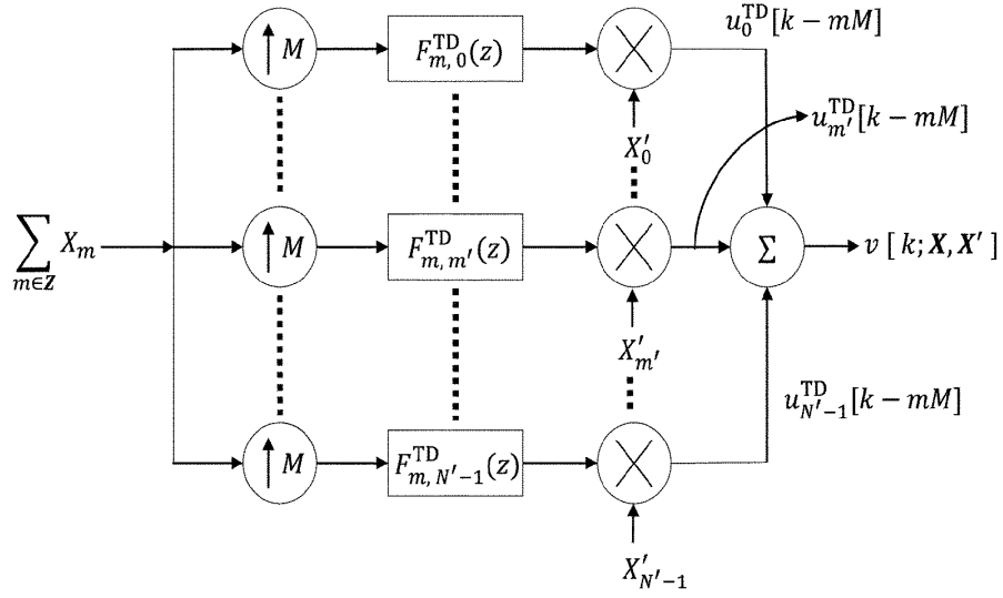
SFB for signature v[k; \mathbf{X}, \mathbf{X}']
