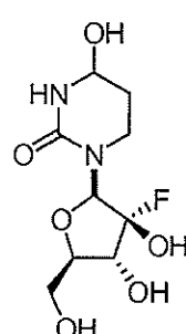
Compound 12
