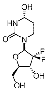
Compound 1a.
