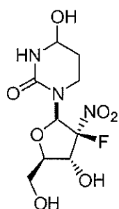
Compound 8
