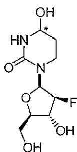
Compound 2
