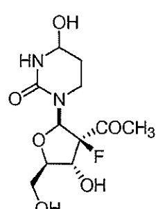
Compound 21
