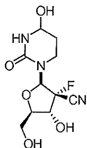
Compound 7
