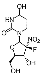
Compound 8
