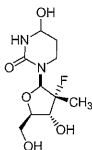
Compound 5
