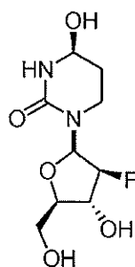
Compound 2b.
