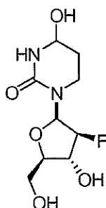
Compound 2
