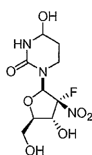
Compound 9
