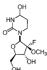
Compound 18
