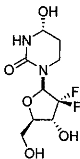
Compound 1a.
