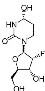
Compound 3a
