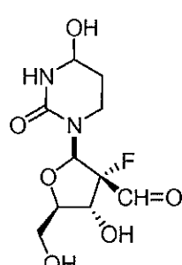
Compound 15
