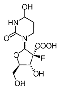
Compound 17
