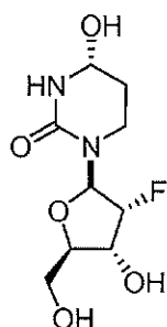
Compound 3a.
