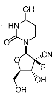
Compound 6
