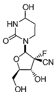
Compound 7
