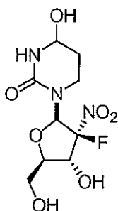
Compound 8
