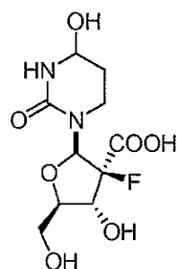
Compound 17
