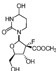
Compound 22
