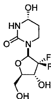
Compound 1a.
