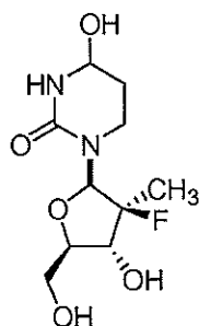
Compound 4
