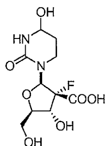
Compound 16
