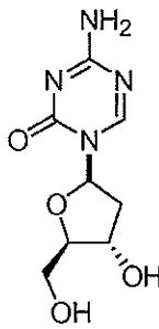
5-aza-2'-deoxycytidine (decitabine)
