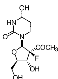
Compound 21
