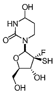
Compound 10
