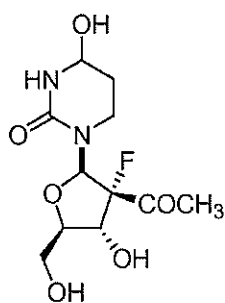
Compound 20
