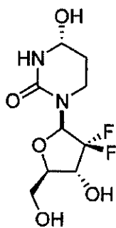
Compound 1a.
