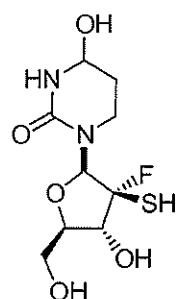
Compound 10
