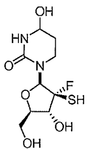
Compound 10
