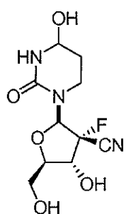
Compound 7
