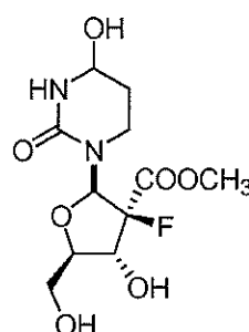
Compound 23
