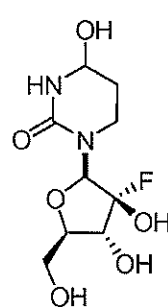
Compound 12
