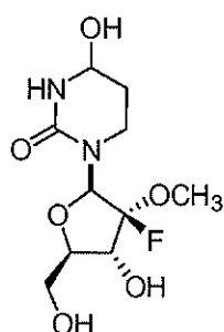
Compound 19
