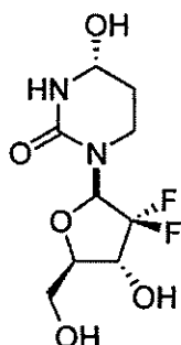
Compound 1a.
