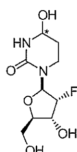
Compound 3
