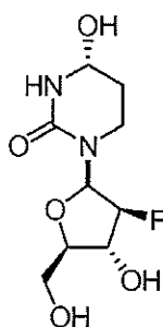
Compound 2a.
