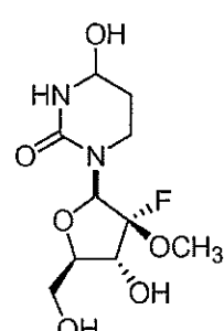
Compound 18
