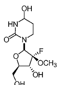
Compound 18
