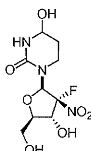
Compound 9
