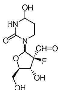
Compound 14
