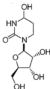
Tetrahydrouridine (THU)
