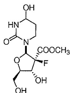
Compound 23
