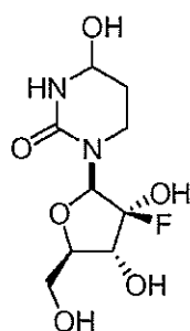
Compound 13
