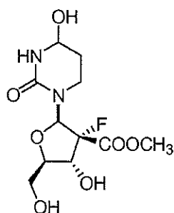
Compound 22
