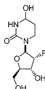
Compound 3
