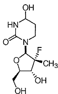
Compound 5
