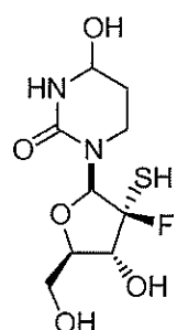
Compound 11
