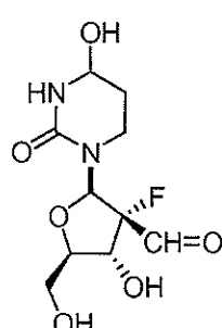
Compound 15
