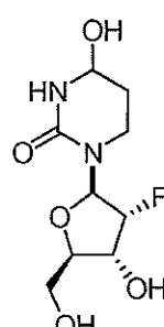
Compound 3
