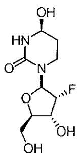
Compound 3b.
