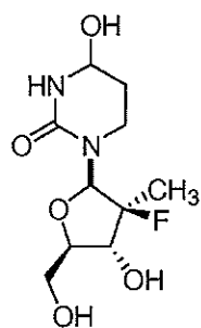
Compound 4
