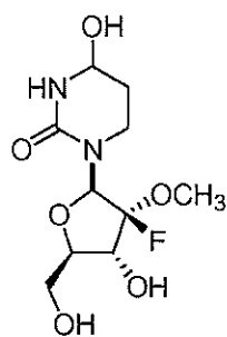
Compound 19
