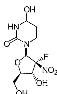
Compound 9
