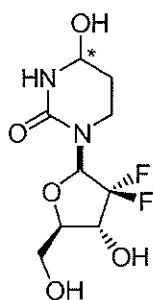
Compound 1
