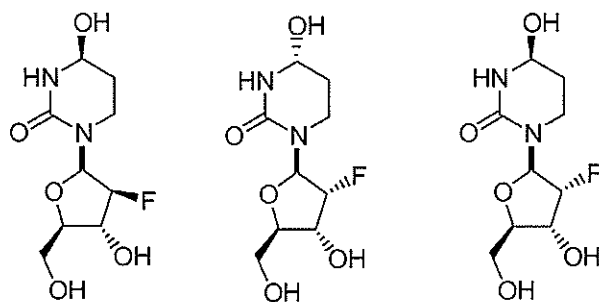
Compound 2b
