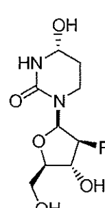
Compound 2a
