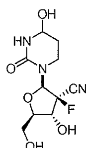
Compound 6
