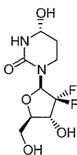
Compound 1a
