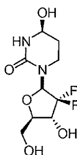
Compound 1b.
