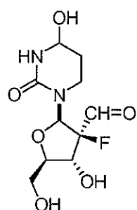
Compound 14
