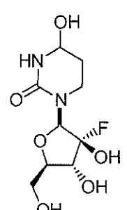
Compound 12
