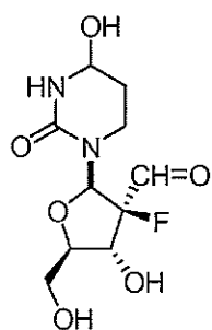
Compound 14
