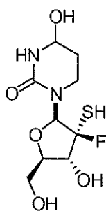
Compound 11
