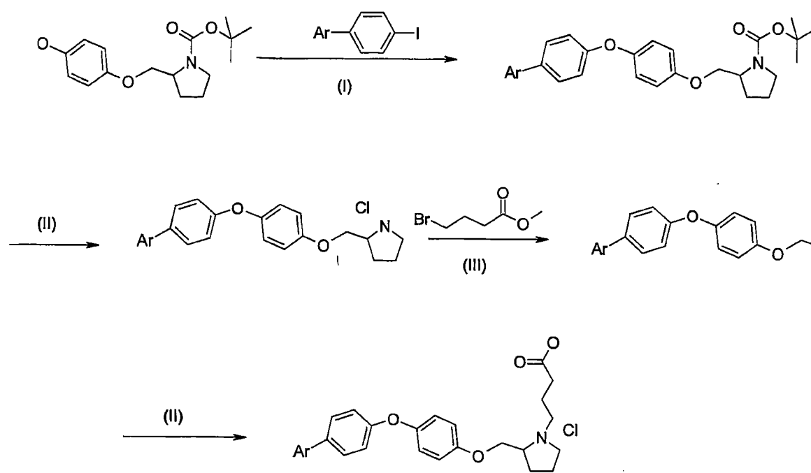
Scheme XV: (I) Cs 2 CO 3 /(CH 3 ) 2 NCH 2 CO 2 H, CuI/dioxane/98 °C, (II) HCl, dioxane, (III) K 2 CO 3 , DMF
