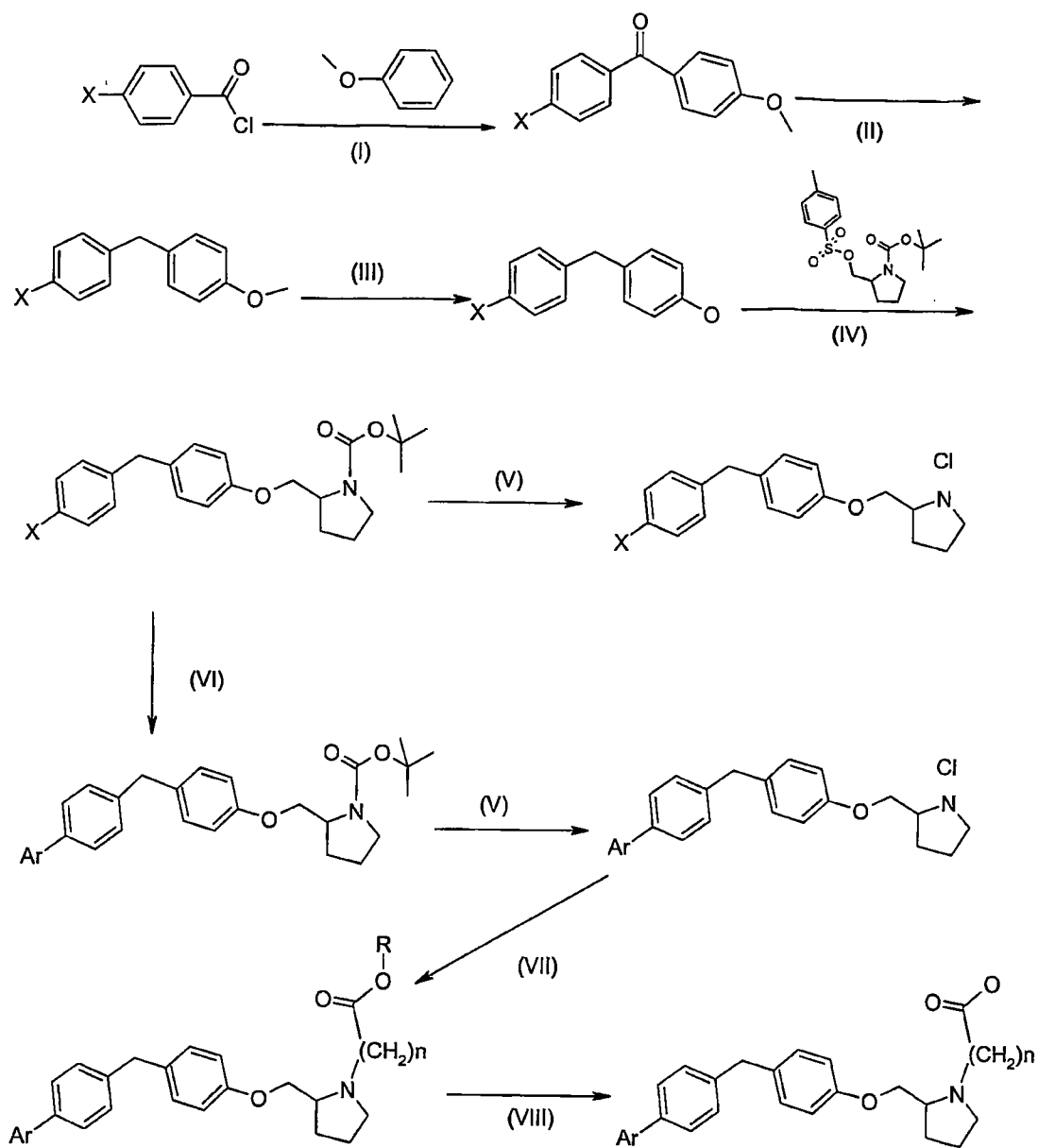
Scheme X: (I) \text{AlCl}_3 , nitrobenzene, (II) \text{Et}_3\text{SiH} , TFA, (III) \text{BBr}_3 , \text{CH}_2\text{Cl}_2 , (IV) \text{NaH} , DMF, (V) \text{HCl} , dioxane, (VI) \text{ArE} \text{Pd}(\text{OAc})_2/\text{PPh}_3/\text{CsCO}_3 , DME/EtOH/ \text{H}_2\text{O} , (VII) \text{Br}(\text{CH}_2)_n\text{CO}_2\text{R} , base, (VIII) \text{NaOH} or \text{HCl} .
