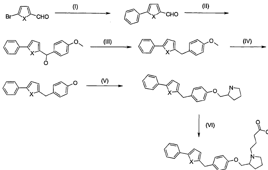
Scheme XXII: (I) \text{ArB(OH)}_2 , Pd/C, i-PrOH/H 2 O, reflux, (II) ArBr, n-BuLi, -78°C, THF, (III) Et 3 SiH, TFA, (IV) BBr 3 , (V) NaH, pyrrolidine tosylate, DMF, (VI) alkyl halide, K 2 CO 3 , DMF
