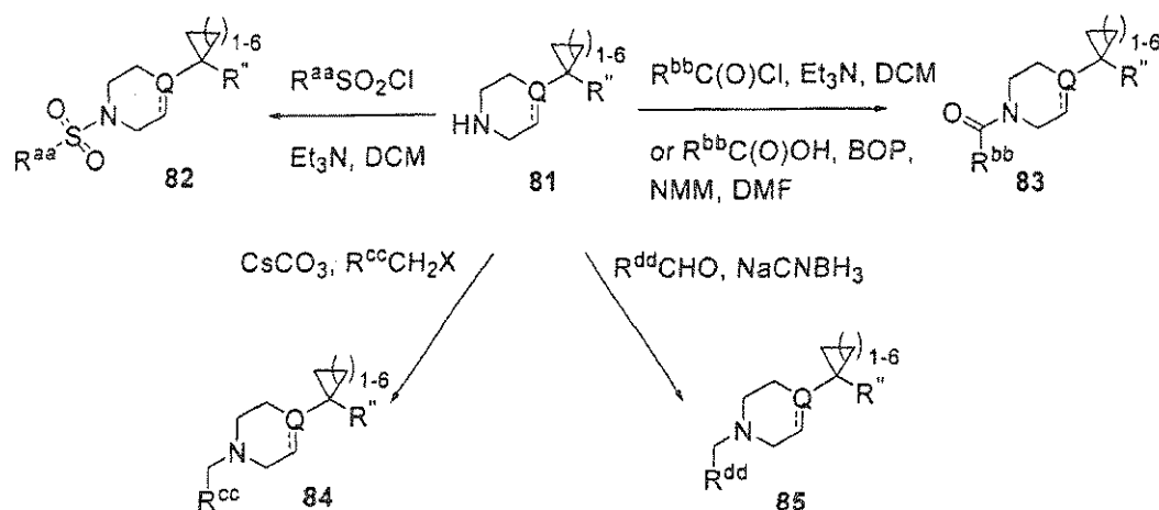
Scheme 22
