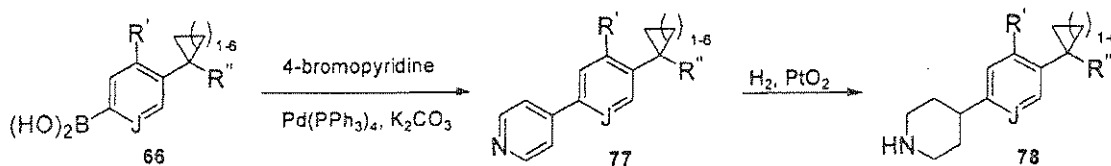
Scheme 20
