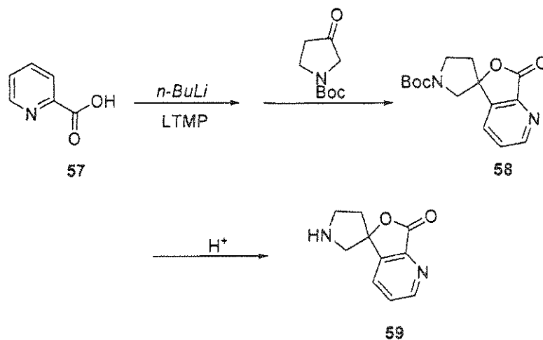
Scheme 15
