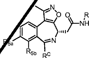
[00105] Table 3. Exemplary Compounds of Formula V.
