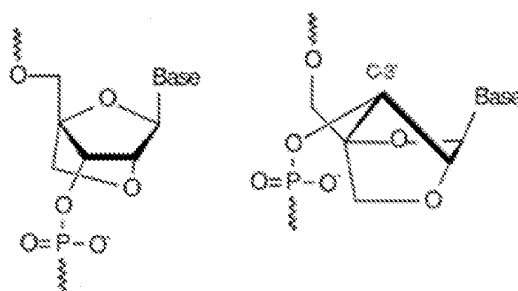
LNA (Locked Nucleic Acids)
