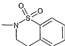
3,4-dihydro-2H-benzo[e][1,2]thiazine-1,1-dioxide-2-yl
