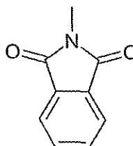
phthalimidyl
