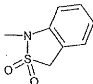
1,3-dihydro-benzo[c]isothiazole-2,2-dioxide-1-yl
