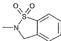
2,3-dihydro-tenzo[d]isothiazole-1,1-dioxide-2-yl
