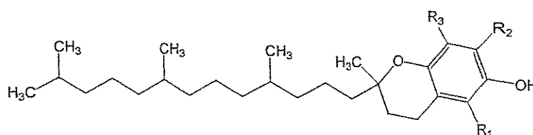
Tocopherol
