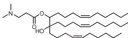
Compound 31,
