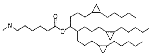
Compound 79,
