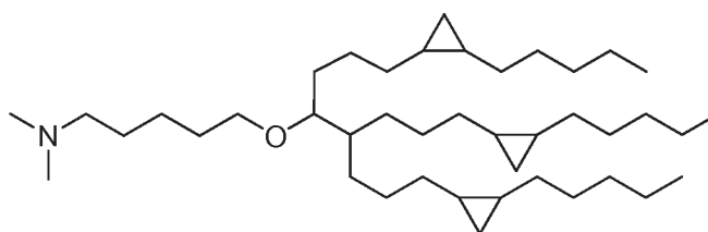
Compound 90.
