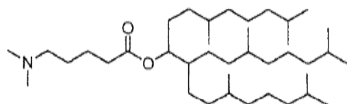
Compound 71,
