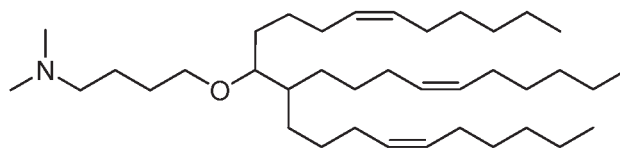
Compound 62,
