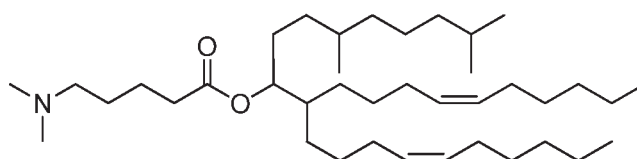
Compound 74,
