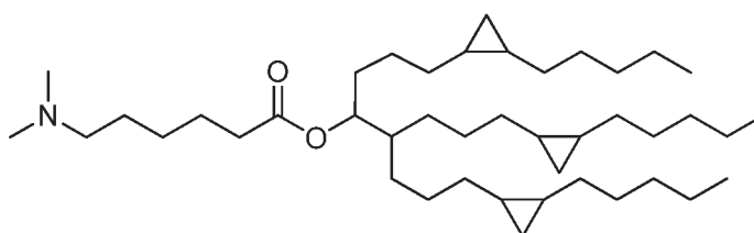
Compound 79,
