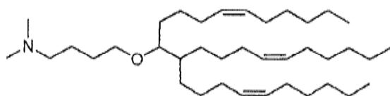
Compound 62,
