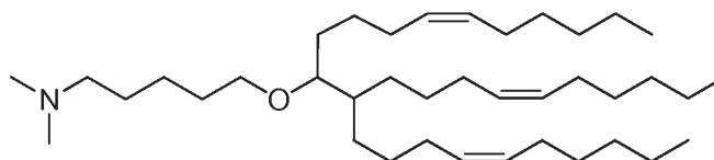
Compound 76,
