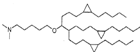
Compound 90.
