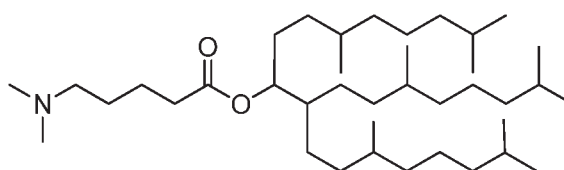
Compound 71,
