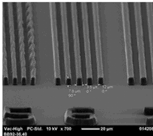
6µm Lines from a 9.8µm Film Dose: 800mJ/cm 2 ; PEB: 3min@105°C
