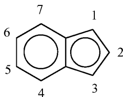
Indenyl
