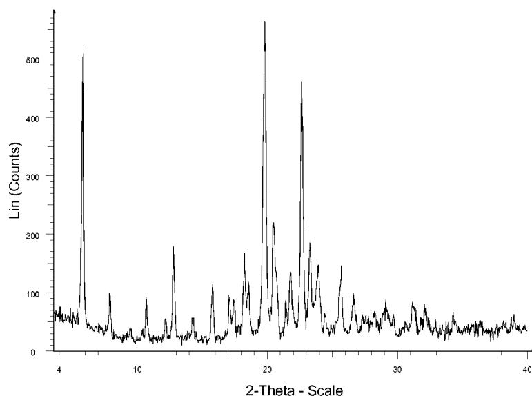
FIG. 1. X-ray powder diffraction pattern of Example 109-B.
