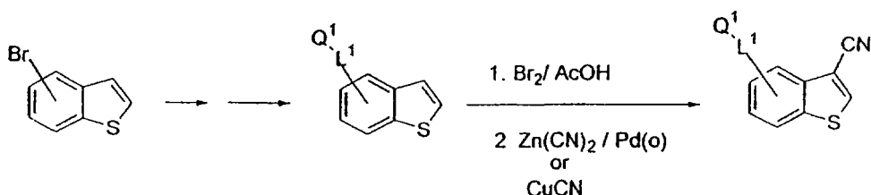
Scheme 7
