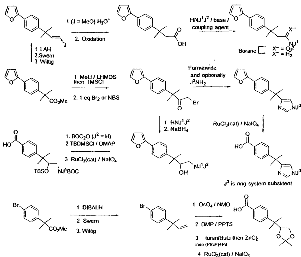
Scheme 10
