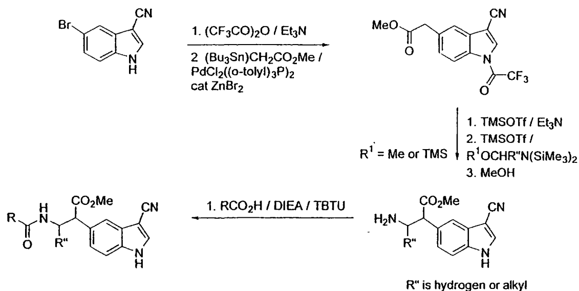
Scheme 11
