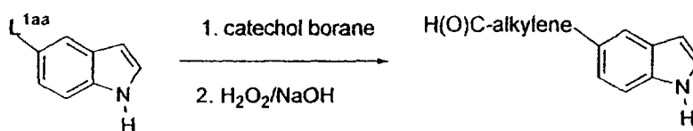
Scheme 5
