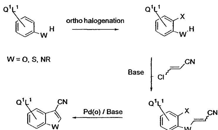
Scheme 8
