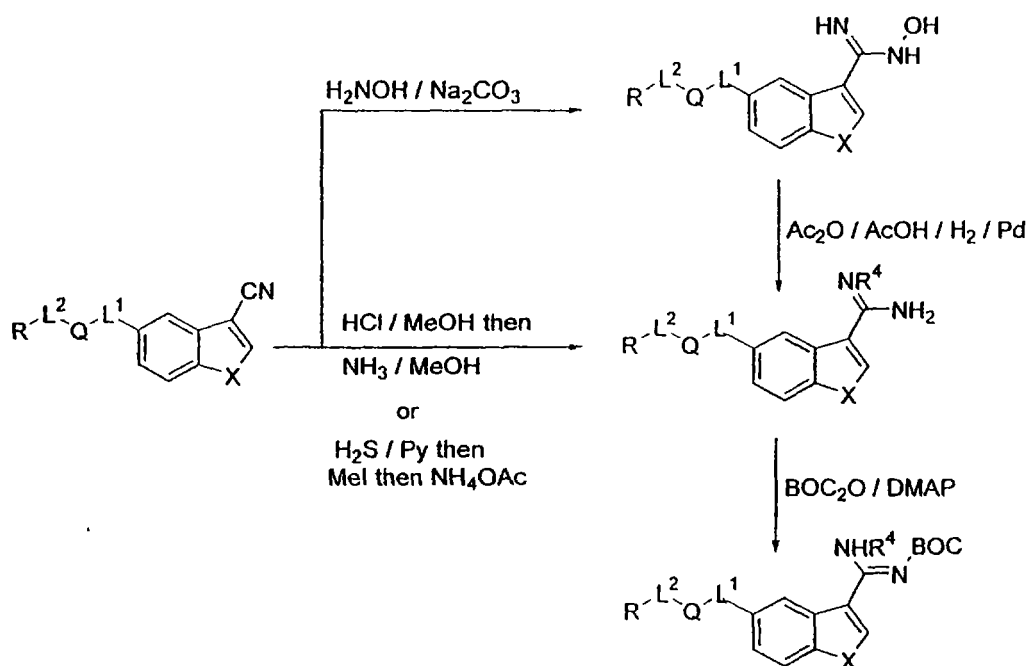
Scheme 12
