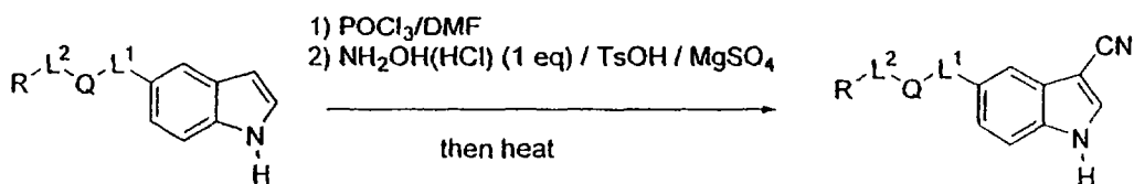
Scheme 6
