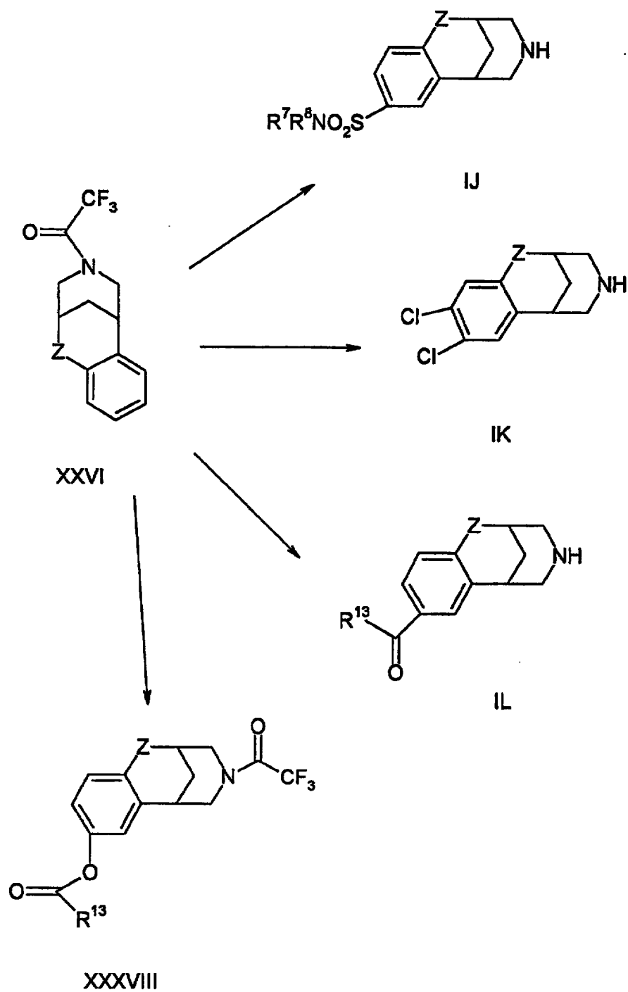
SCHEME 12
