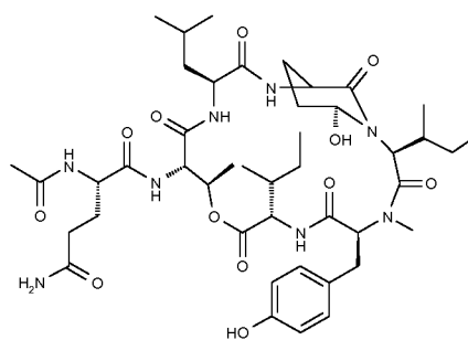
Formula (XII)
