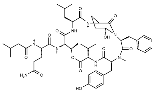
Formula (VIII)
