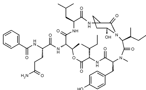
Formula (XIII)
