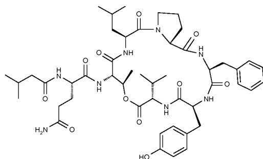
Formula (X)
