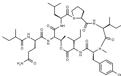
Formula (XIV)
