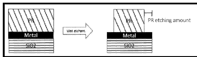
FIG. 1. Photoresist Removal
