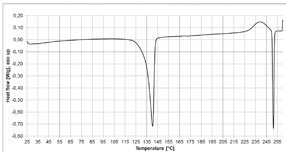
Figure 4. DSC plot of the compound of the formula (IIa).
