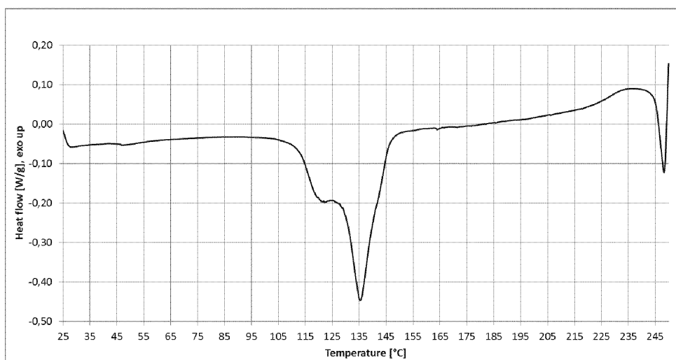
Figure 6. DSC plot of the compound of the formula (IIc).
