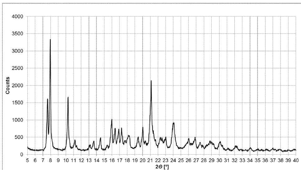
Figure 2. XRPD plot of the compound of the formula (IIb).
