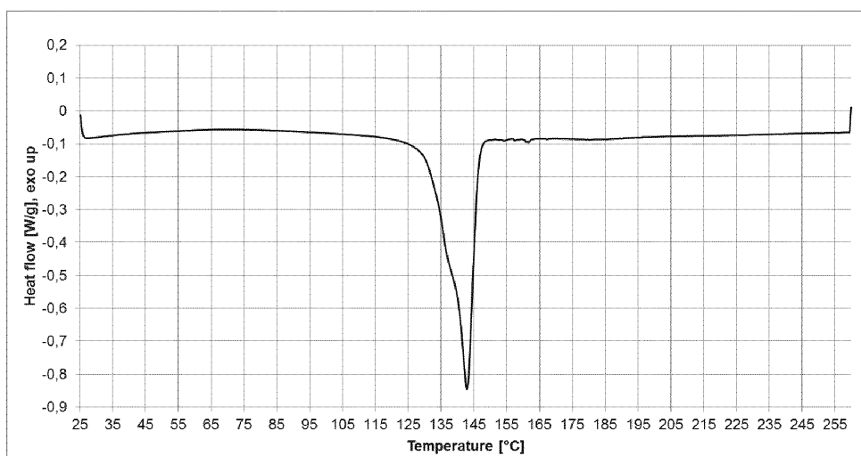
Figure 5. DSC plot of the compound of the formula (IIb).
