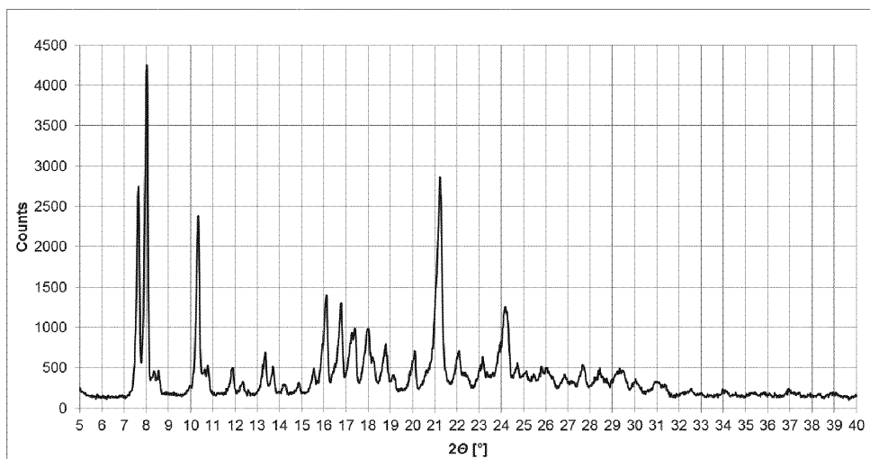
Figure 1. XRPD plot of the compound of the formula (IIa).
