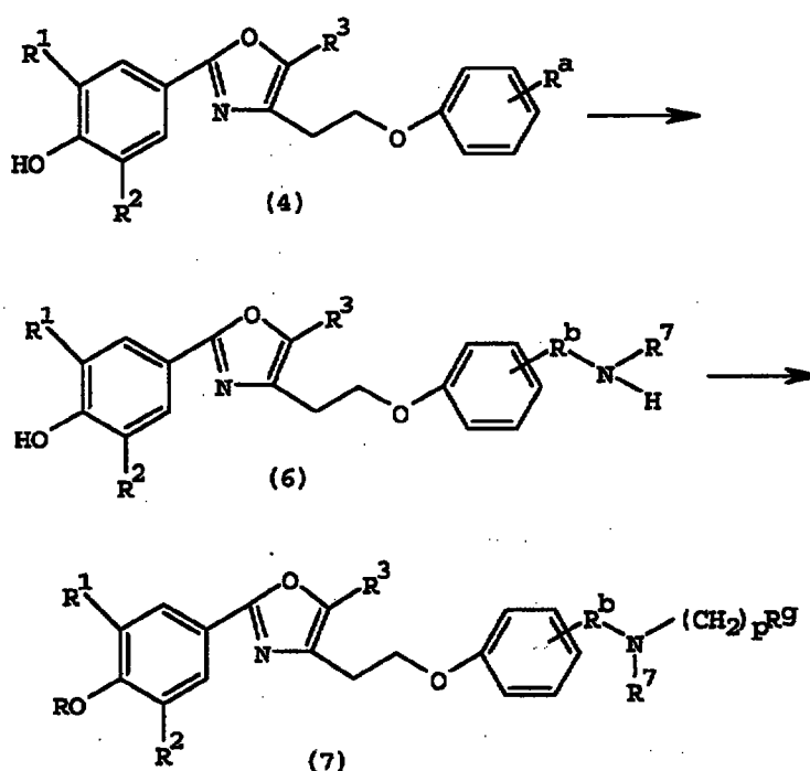
Scheme I(b)
