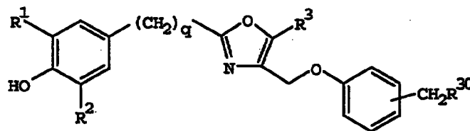
(XXI)
