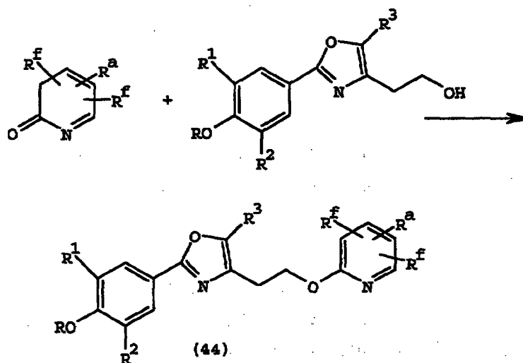
Scheme X
