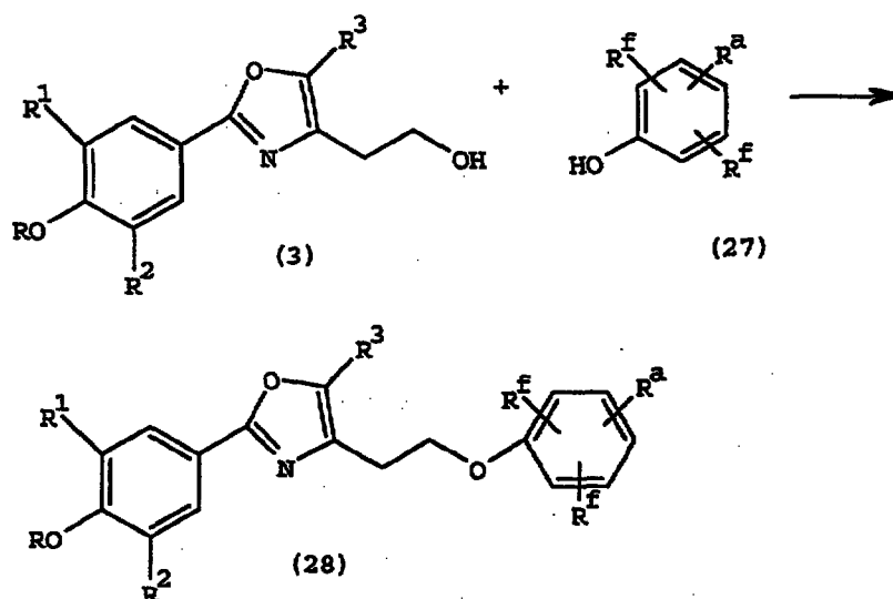
Scheme IV
