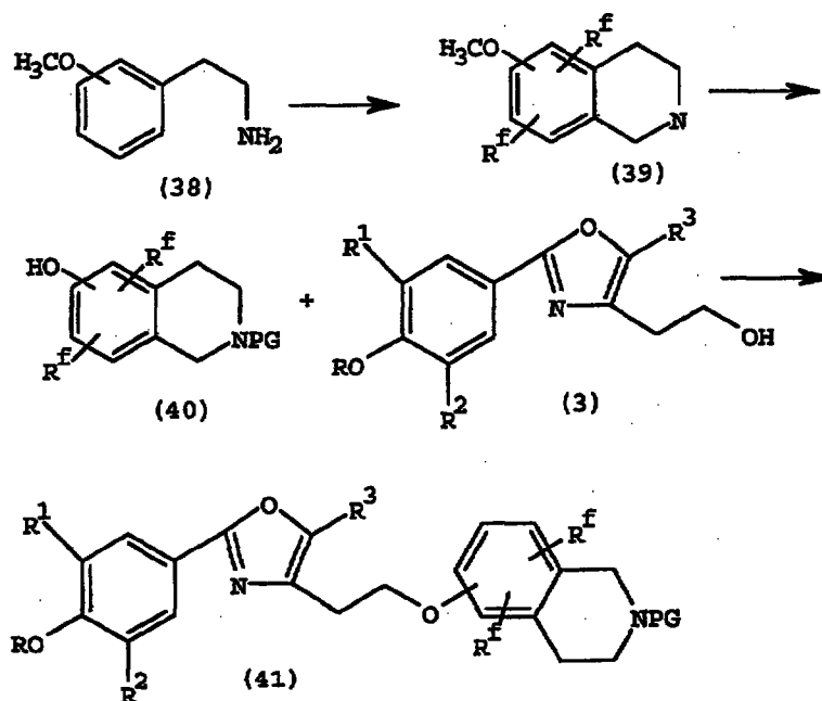
Scheme IX (a)
