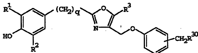
(XXI)
