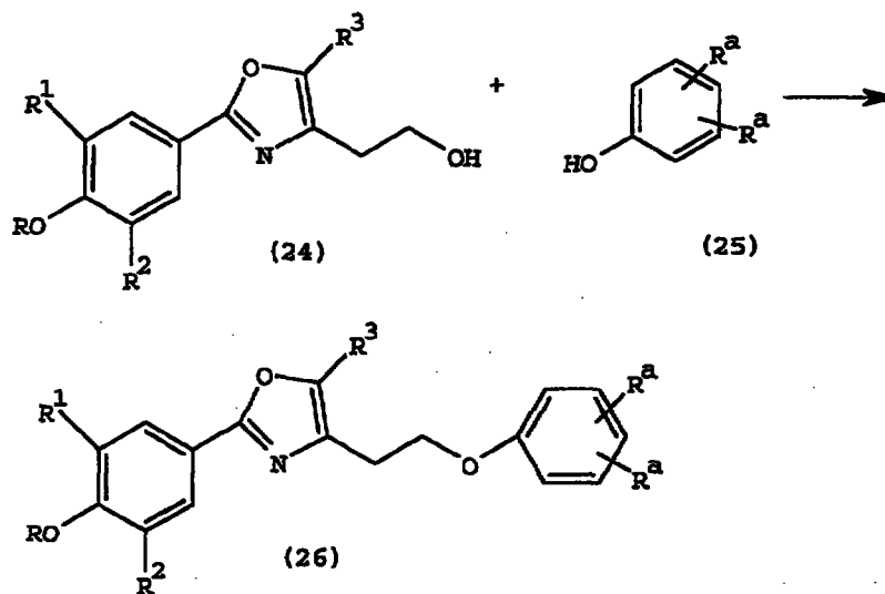
Scheme III
