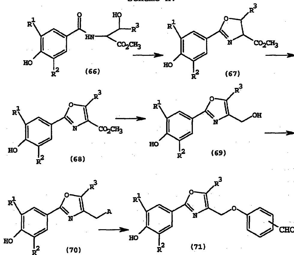
Scheme XV
