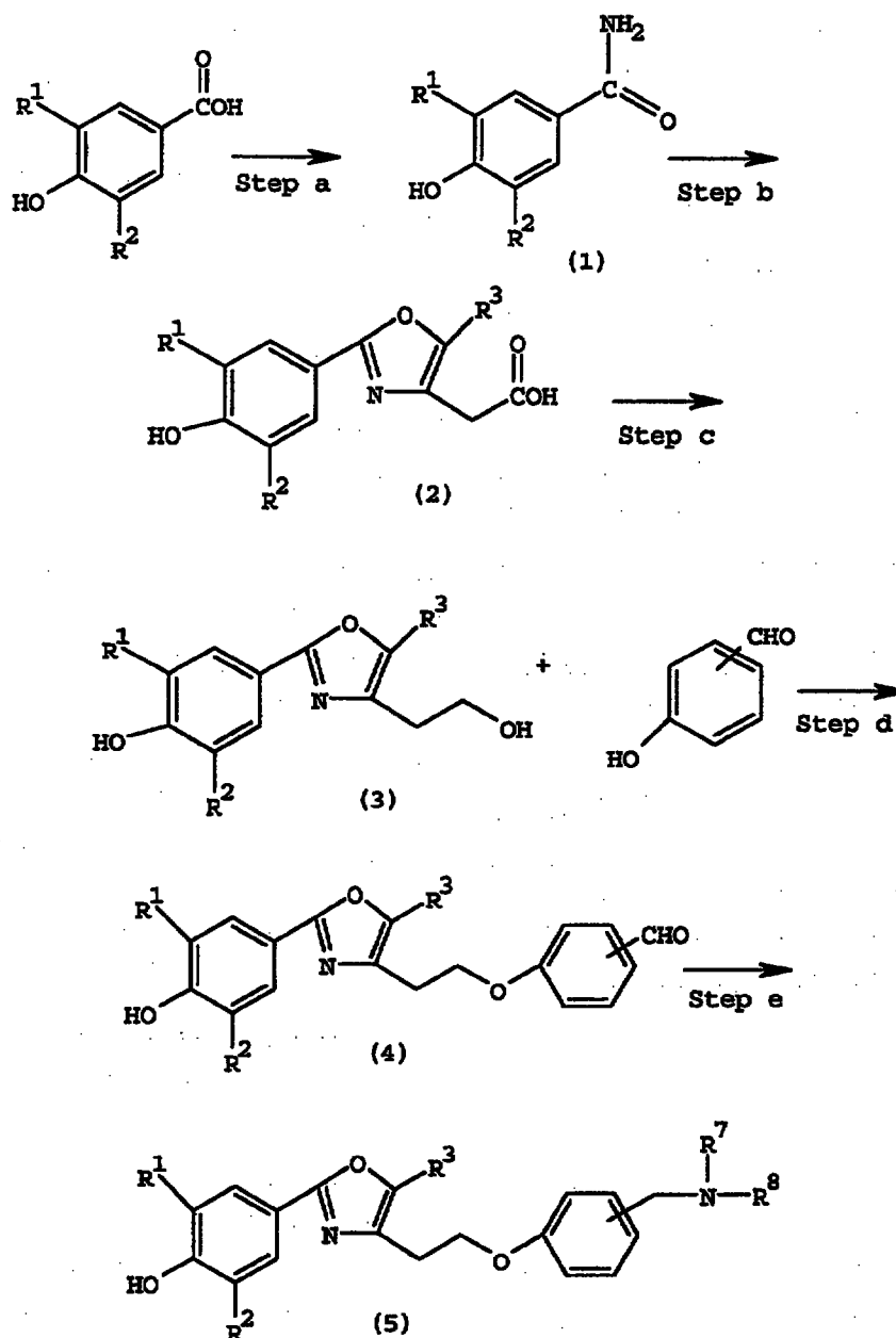
Scheme I(a) (1)
