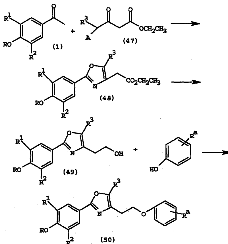
Scheme XII
