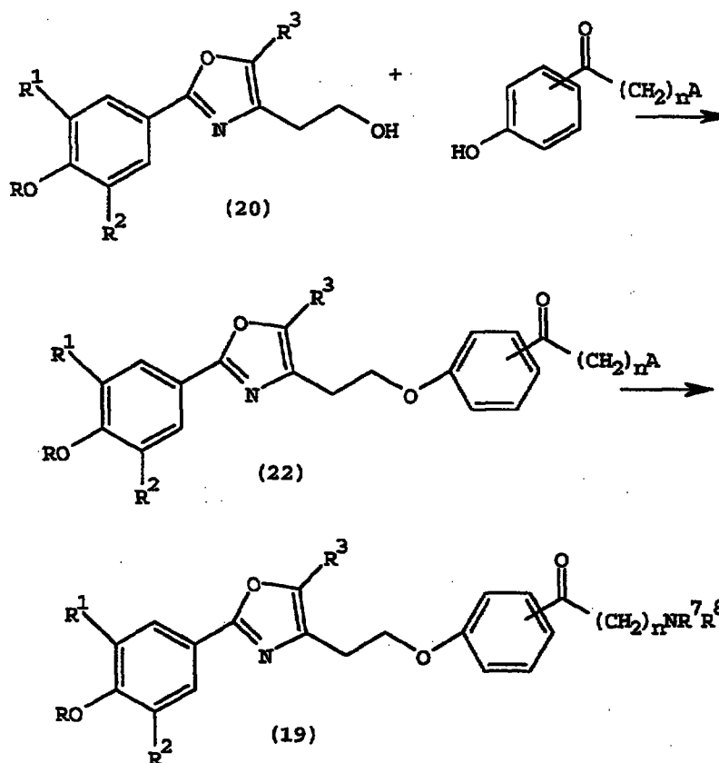
Scheme II.
