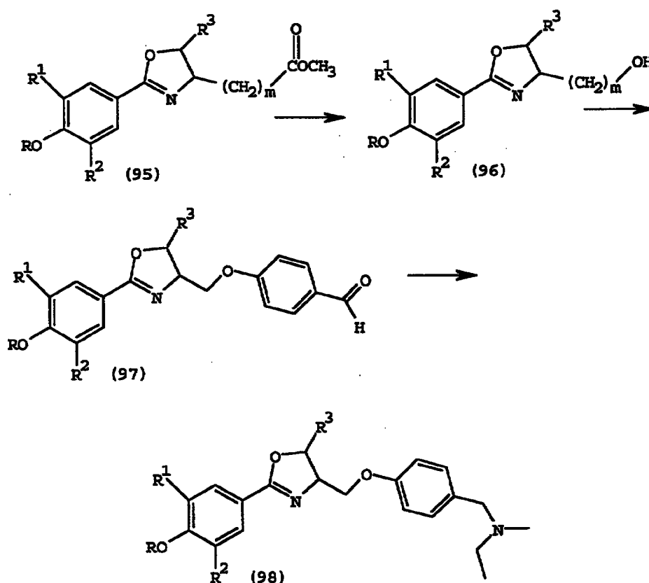
Scheme XXI
