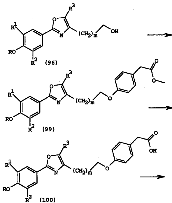
Scheme XXII
