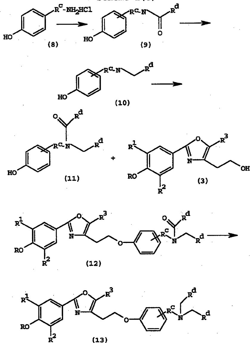
Scheme I(c)
