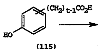
Scheme I(a) (3)
