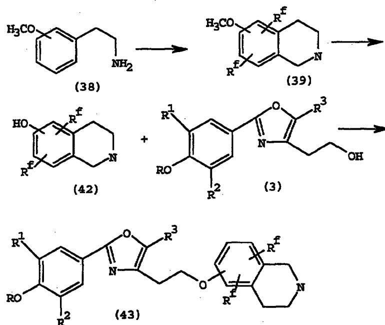
Scheme IX(b)
