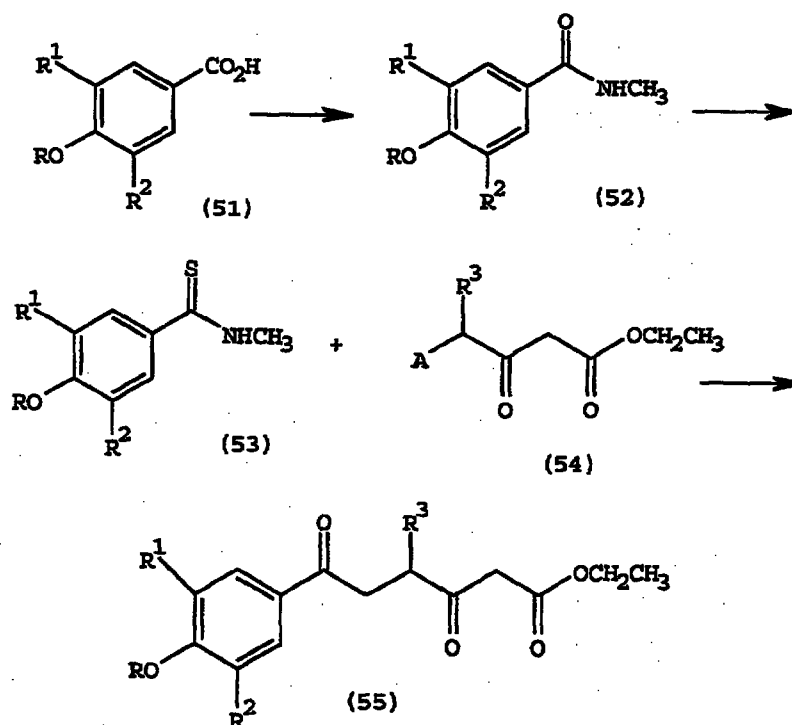
Scheme XIII
