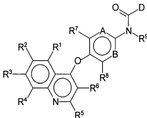
formula (I)
