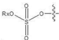
[Chemical Formula 2-9]
