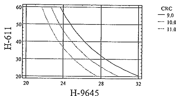
Figure 3. Contours of estimated response surfaces for CRC rating
