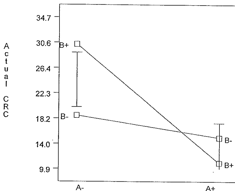
Figure 2. Interaction of A:H-9645 and B:H-611
