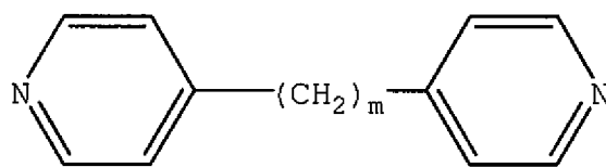
Structure (IIe)
