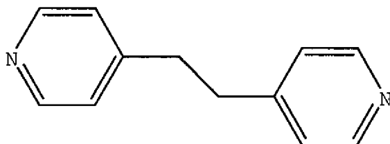
Structure (IIf)
