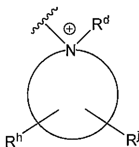
(2B)
