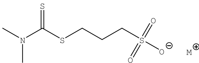
Structure (5)
