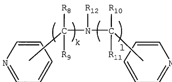
Structure (Ic)
