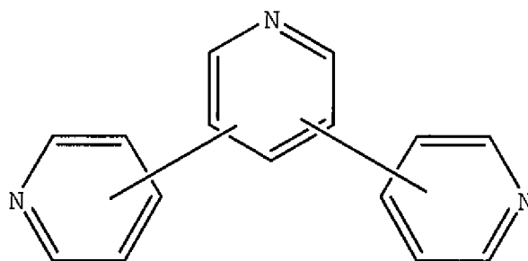
Structure (Id)
