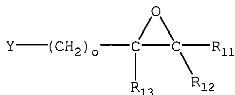
Structure (IIIc)
