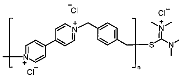
Structure D
