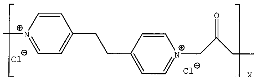
Structure (X)
