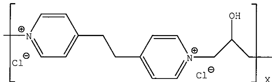
Structure (XI)
