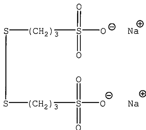
Structure (3)
