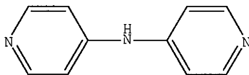
dipyridin-4-ylamine
