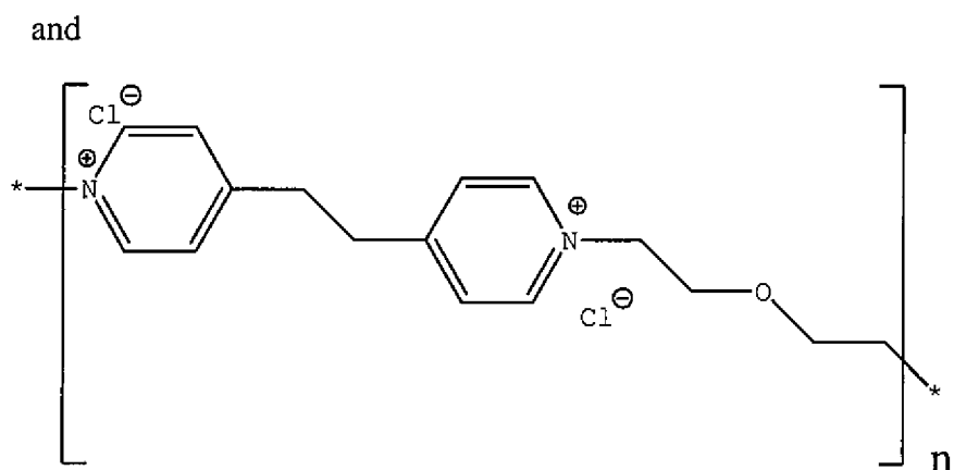
Structure (VIII)
