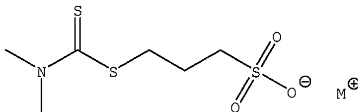
Structure (5)
