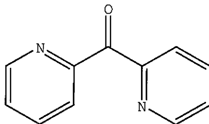
2,2'-dipyriddy ketone
