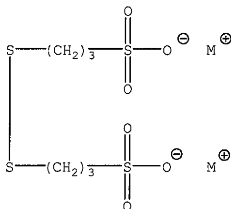
Structure (2)
