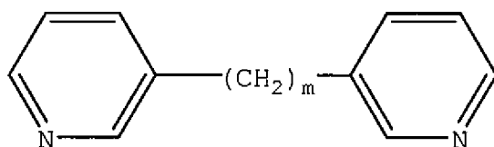
Structure (IIc)
