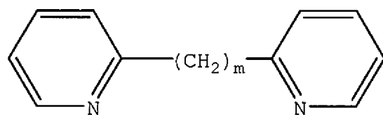
Structure (IIb)
