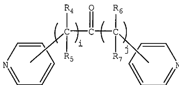
Structure (Ib)
