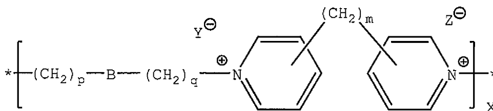
Structure (IV)
