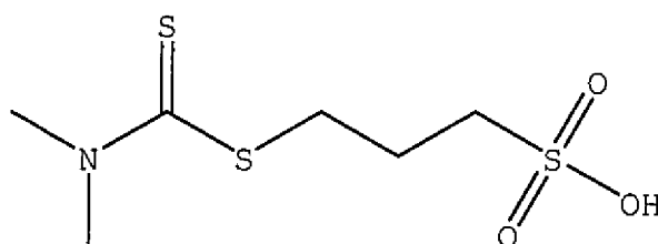
Structure (16)
