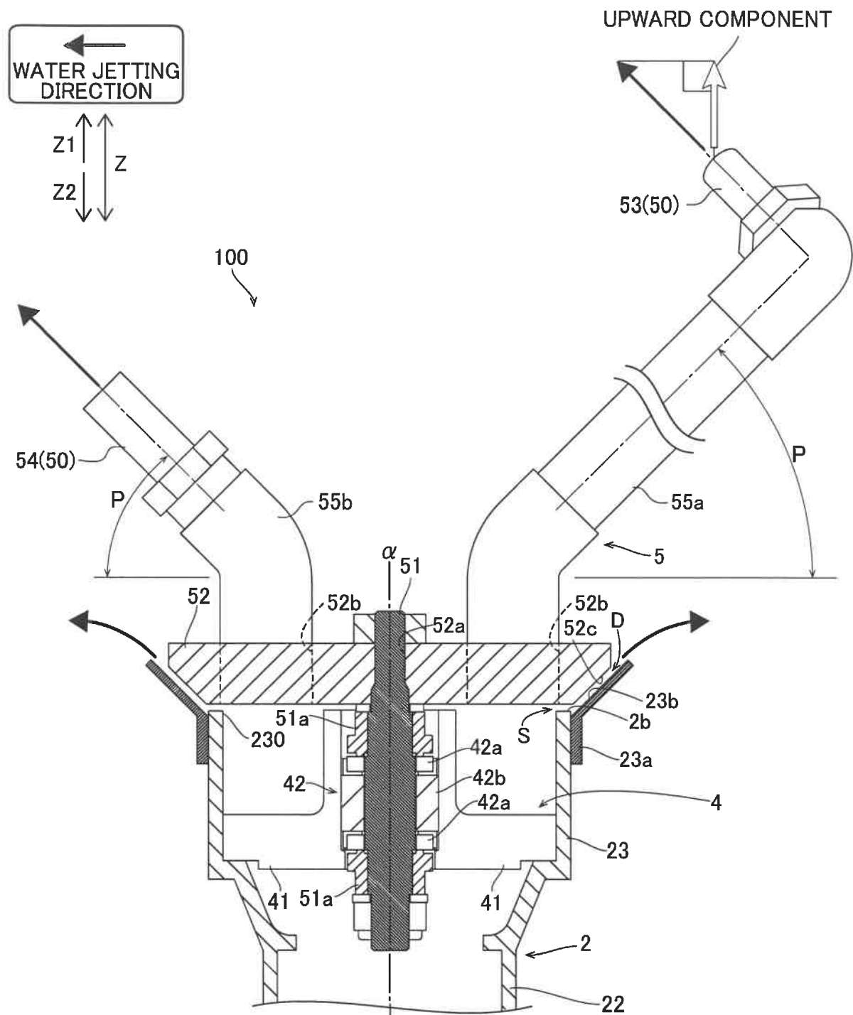
FIG.3 500-500 SECTION
