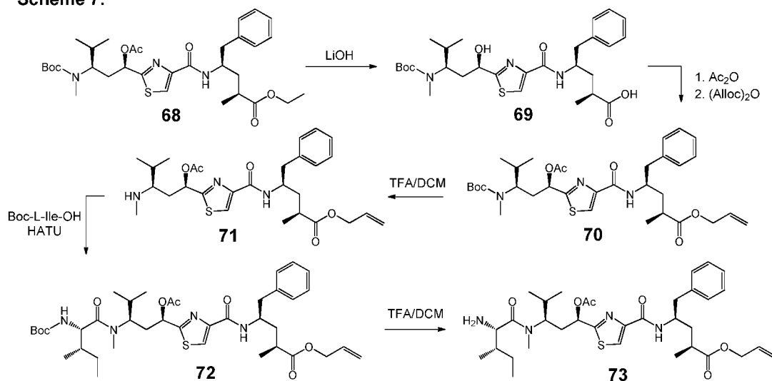
Scheme 7.
