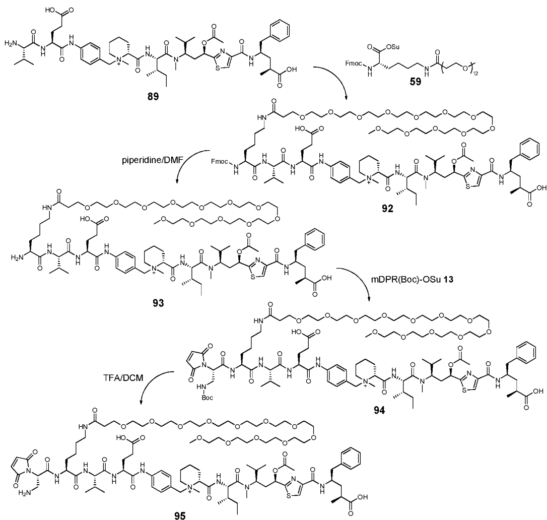
Scheme 11.
