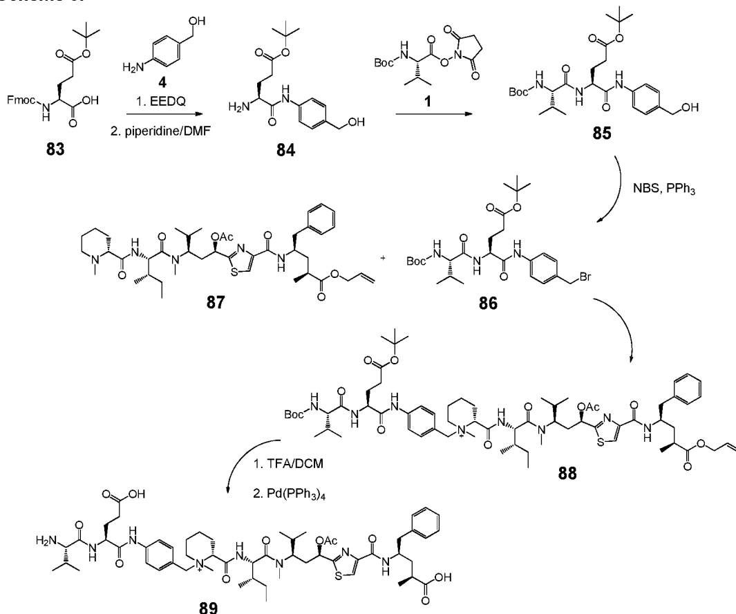
Scheme 9.
