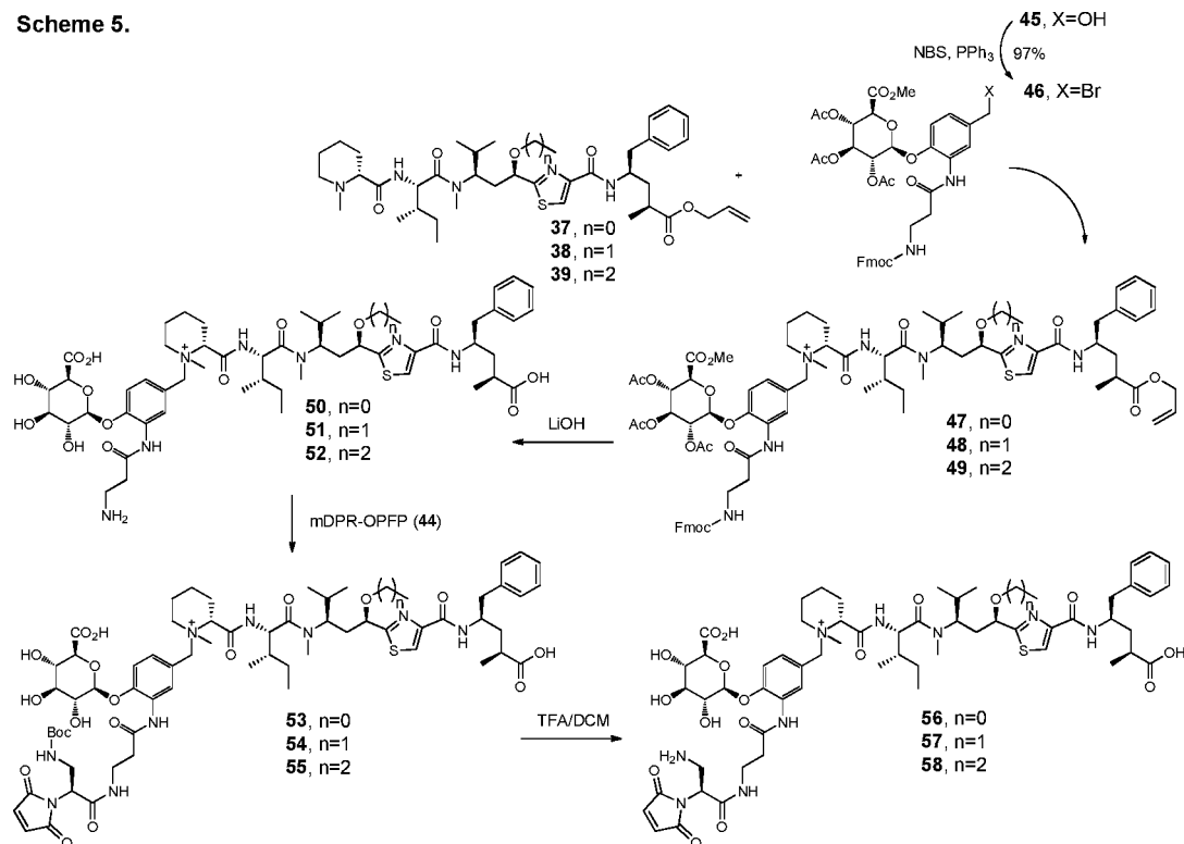
Scheme 5.
