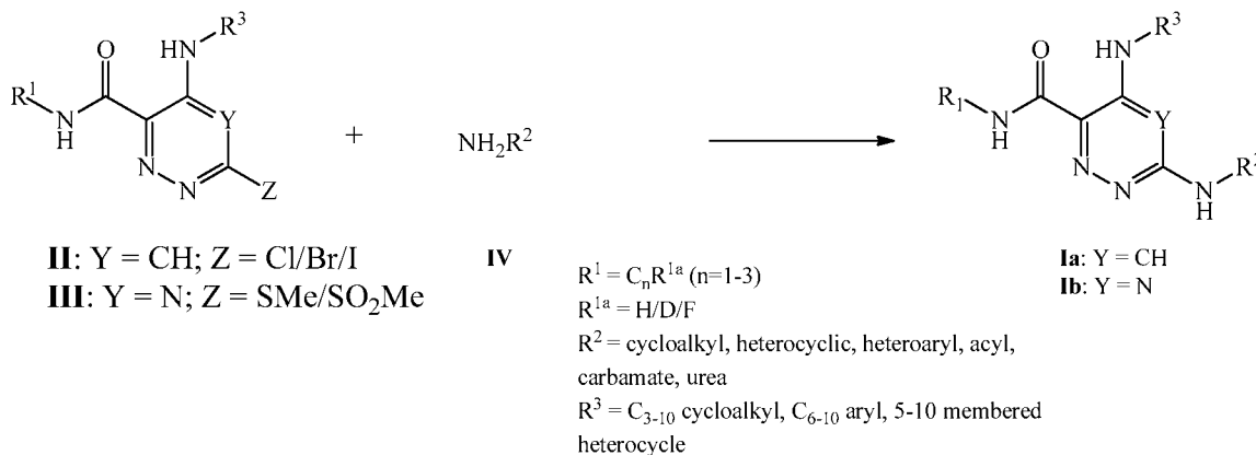
Scheme 1. Coupling of II/III with amine IV
