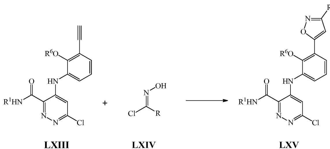
Scheme 17. Synthesis of LXV
