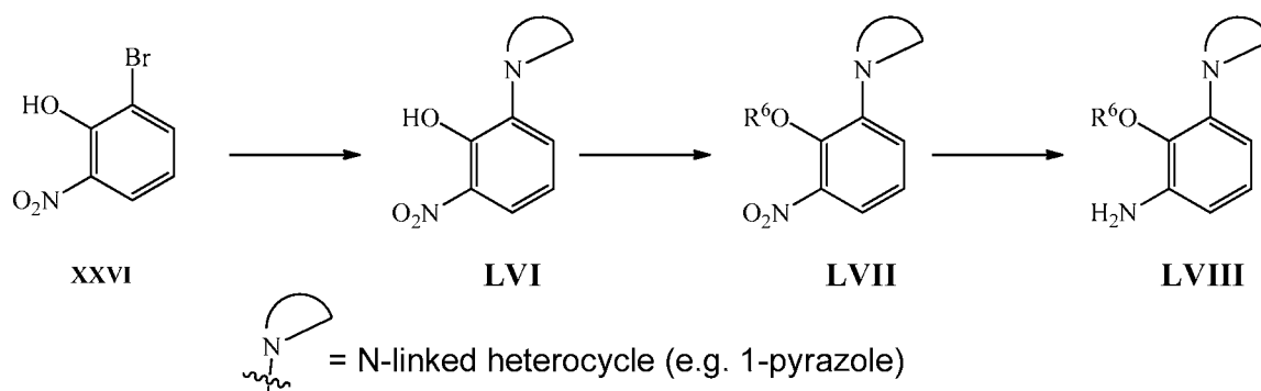
Scheme 15. Synthesis of anilines LVIII (variant of XII )
