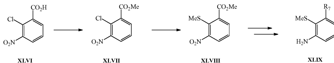
Scheme 13. Synthesis of thioanilines XLIX
