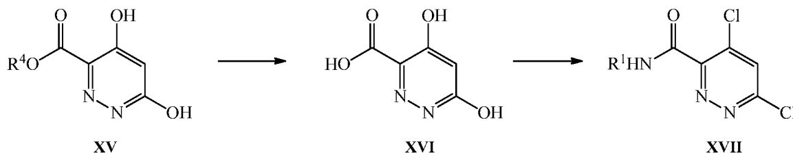
Scheme 6. Preparation of XVII
