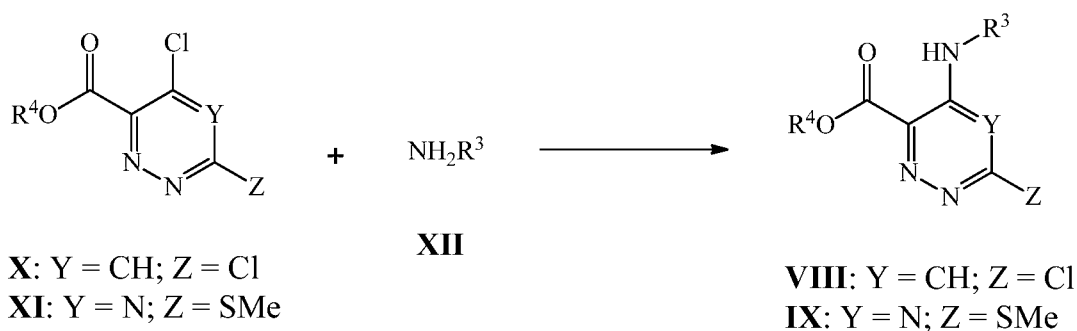
Scheme 4. Coupling of chlorides X/XI with amine XII
