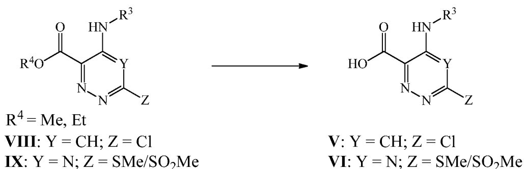
Scheme 3. Saponification of esters VIII/IX
