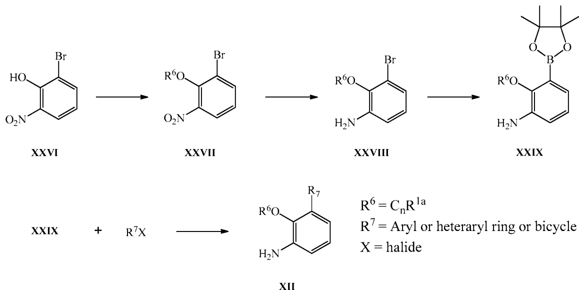
Scheme 10. Synthesis of anilines XII
