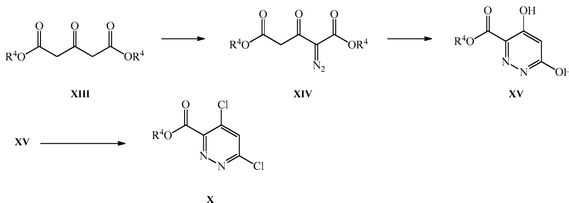
Scheme 5. Preparation of X
