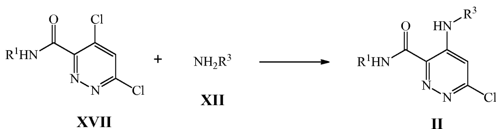
Scheme 7. Preparation of II
