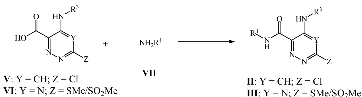
Scheme 2. Coupling of carboxylic acids V / VI with amine VII
