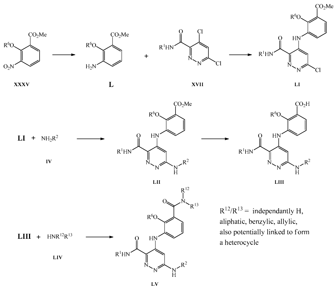
Scheme 14. Synthesis of final compounds LV
