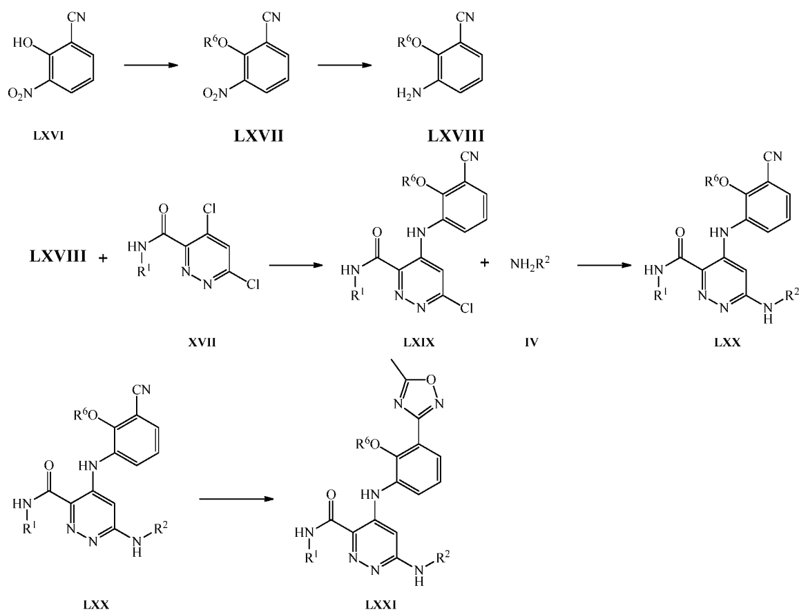
Scheme 18. Synthesis of LXXI
