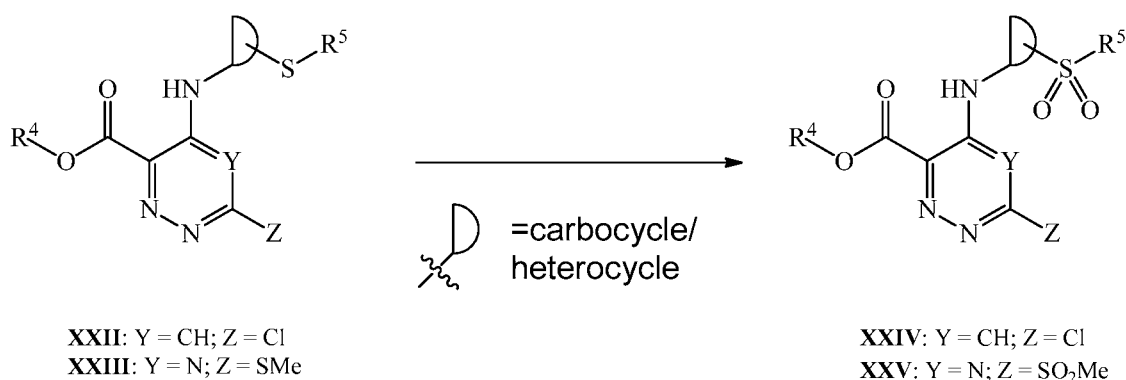
Scheme 9. Oxidation of pendant sulfides
