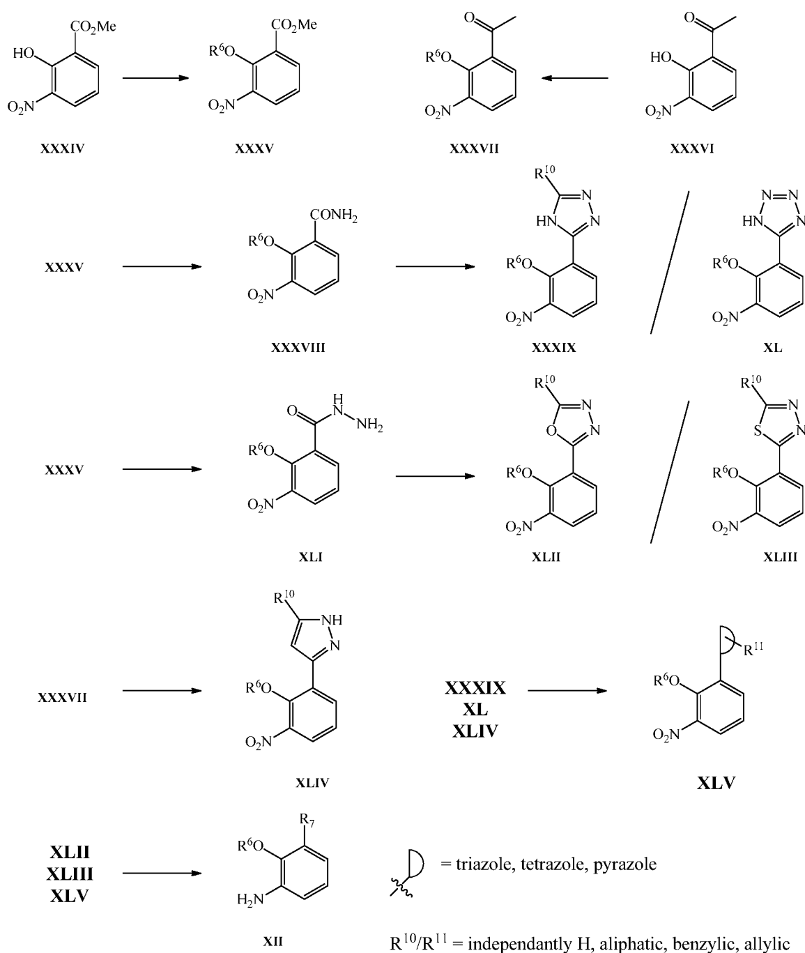
Scheme 12. Alternate synthesis of anilines XII
