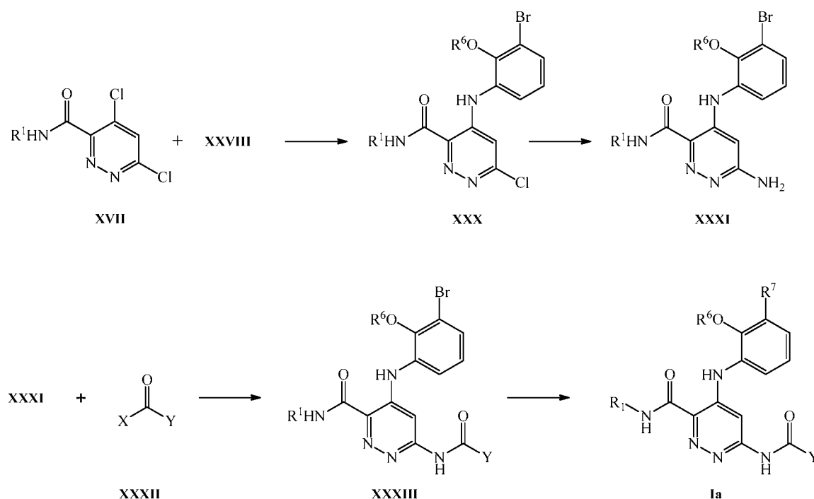
Scheme 11. Alternative preparation of I
