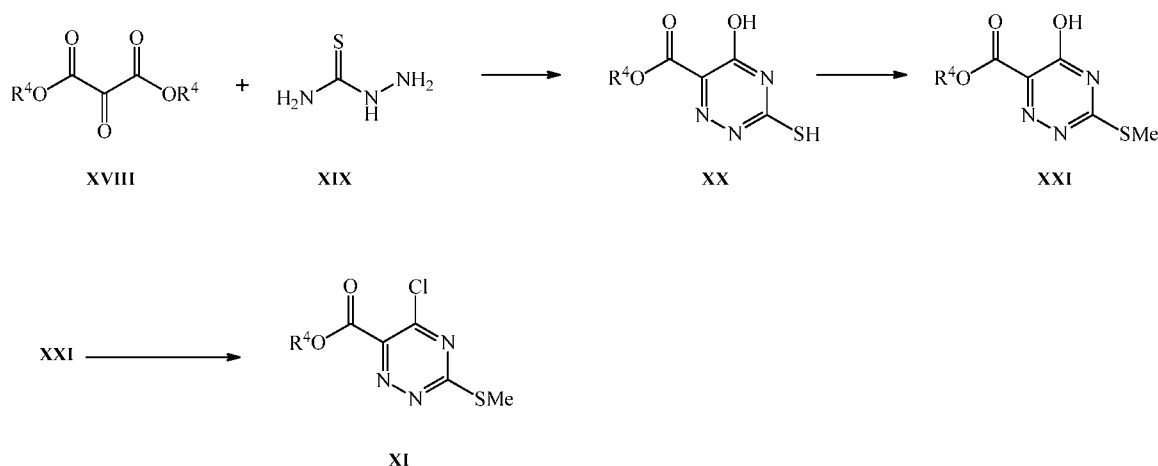
Scheme 8. Preparation of XI
