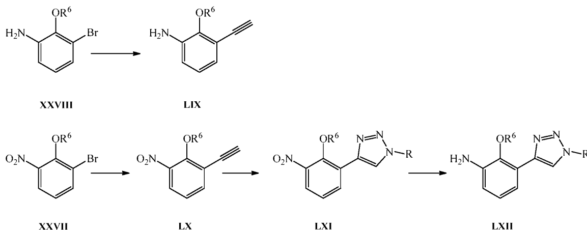
Scheme 16. Synthesis of anilines LIX and LXII (variants of XII )
