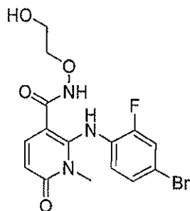
2-(4-bromo-2-fluorophenylamino)-N-(2-hydroxyethoxy)-1-methyl-6-oxo-1,6-dihydropyridine-3-carboxamide
