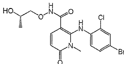
(S)-2-(4-bromo-2-chlorophenylamino)-N-(2-hydroxypropoxy)-1-methyl-6-oxo-1,6-dihydropyridine-3-carboxamide
