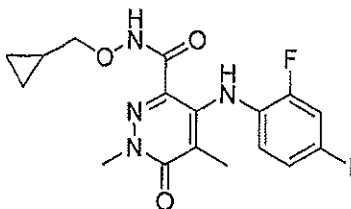
N-(Cyclopropylmethoxy)-4-(2-fluoro-4-iodophenylamino)-1,5-dimethyl-6-oxo-1,6-dihydropyridazine-3-carboxamide
