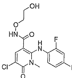
5-chloro-2-(2-fluoro-4-iodophenylamino)-N-(2-hydroxyethoxy)-1-methyl-6-oxo-1,6-dihydropyridine-3-carboxamide
