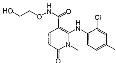
2-(2-chloro-4-iodophenylamino)-N-(2-hydroxyethoxy)-1-methyl-6-oxo-1,6-dihydropyridine-3-carboxamide
