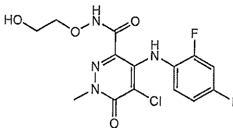
5-Chloro-4-(2-fluoro-4-iodophenylamino)-N-(2-hydroxyethoxy)-1-methyl-6-oxo-1,6-dihydropyridazine-3-carboxamide
