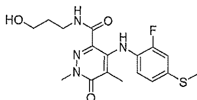
4-(2-Fluoro-4-(methylthio)phenylamino)-N-(3-hydroxypropyl)-1,5-dimethyl-6-oxo-1,6-dihydropyridazine-3-carboxamide
