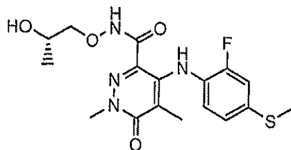
(S)-4-(2-fluoro-4-(methylthio)phenylamino)-N-(2-hydroxypropoxy)-1,5-dimethyl-6-oxo-1,6-dihydropyridazine-3-carboxamide
