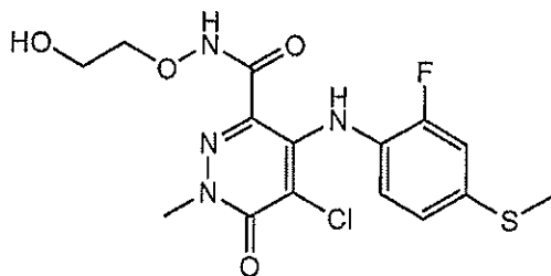
5-Chloro-4-(2-fluoro-4-(methylthio)phenylamino)-N-(2-hydroxyethoxy)-1-methyl-6-oxo-1,6-dihydropyridazine-3-carboxamide
