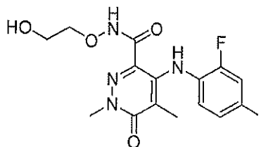
4-(2-Fluoro-4-iodophenylamino)-N-(2-hydroxyethoxy)-1,5-dimethyl-6-oxo-1,6-dihydropyridazine-3-carboxamide
