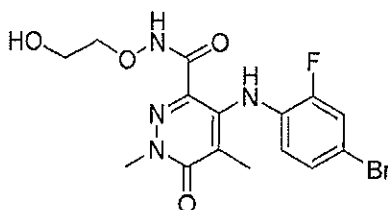
4-(4-Bromo-2-fluorophenylamino)-N-(2-hydroxyethoxy)-1,5-dimethyl-6-oxo-1,6-dihydropyridazine-3-carboxamide
