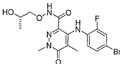
(S)-4-(4-Bromo-2-fluorophenylamino)-N-(2-hydroxypropoxy)-1,5-dimethyl-6-oxo-1,6-dihydropyridazine-3-carboxamide
