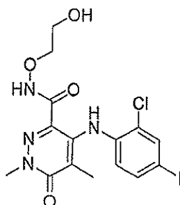
4-(2-chloro-4-iodophenylamino)-N-(2-hydroxyethoxy)-1,5-dimethyl-6-oxo-1,6-dihydropyridazine-3-carboxamide
