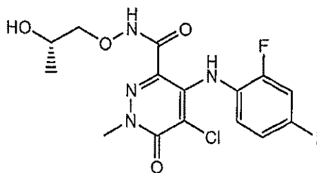
(S)-5-Chloro-4-(2-fluoro-4-iodophenylamino)-N-(2-hydroxypropoxy)-1-methyl-6-oxo-1,6-dihydropyridazine-3-carboxamide
