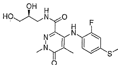
(S)-N-(2,3-Dihydroxypropyl)-4-(2-fluoro-4-(methylthio)phenylamino)-1,5-dimethyl-6-oxo-1,6-dihydropyridazine-3-carboxamide
