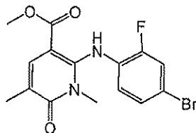
Methyl 2-(4-bromo-2-fluorophenylamino)-1,5-dimethyl-6-oxo-1,6-dihydropyridine-3-carboxylate
