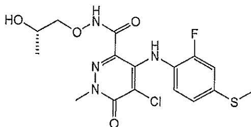
(S)-5-Chloro-4-(2-fluoro-4-(methylthio)phenylamino)-N-(2-hydroxypropoxy)-1-methyl-6-oxo-1,6-dihydropyridazine-3-carboxamide
