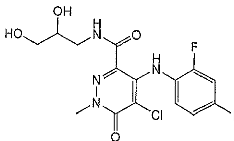
5-Chloro-N-(2,3-dihydroxypropyl)-4-(2-fluoro-4-iodophenylamino)-1-methyl-6-oxo-1,6-dihydropyridazine-3-carboxamide
