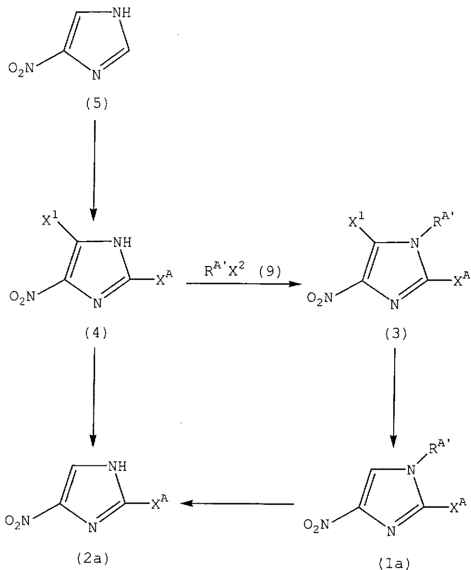
Reaction scheme-3
