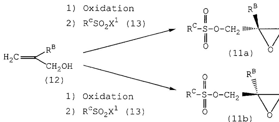
Reaction scheme-5
