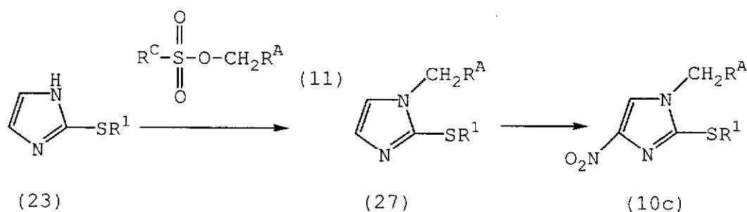
Reaction scheme-9
