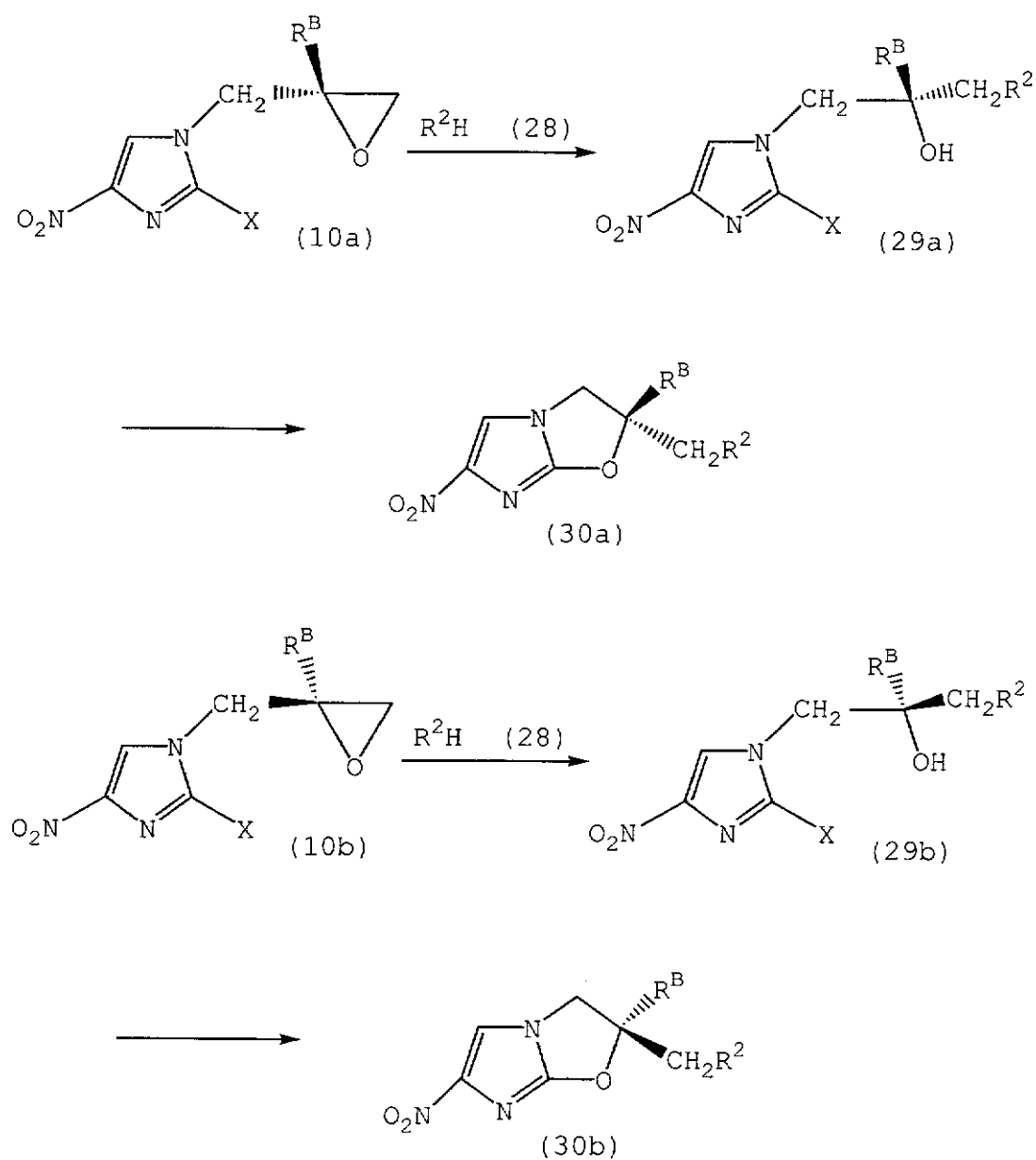
Reaction scheme-12
