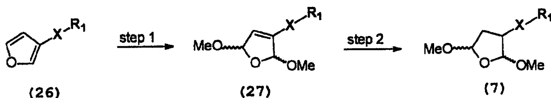
REACTION SCHEME XI
