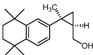
(Compound 9),
