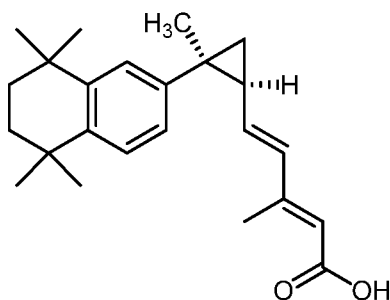
Compound A,
