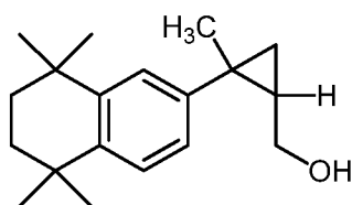
Compound 29
