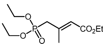
(Compound 12),
