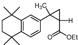
(Compound 33),
