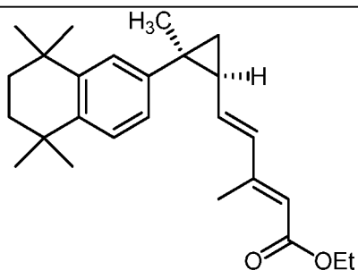
Compound 13
