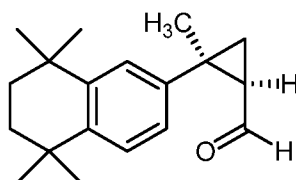
(Compound 11),
