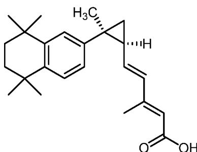
Compound A,
