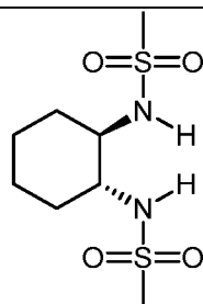
Compound 5
