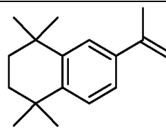
Compound 16
