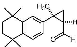
(Compound 11),
