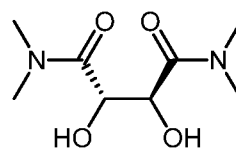
Compound 28
