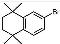
Compound 3
