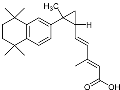
Compound 38,
