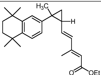
Compound 37
