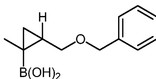
(Compound 21),
