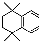
Compound 14
