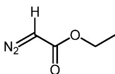
(Compound 17),
