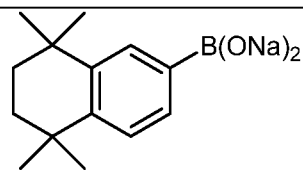
Compound 4
