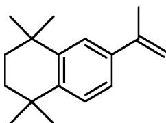
(Compound 16),
