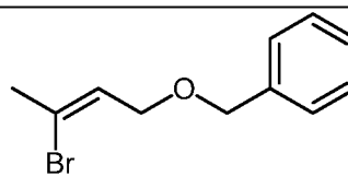
Compound 18
