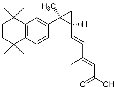
Compound A,
