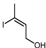
Compound 7
