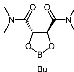
Compound 6
