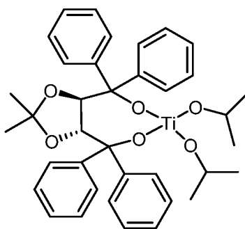
(Compound 39),
