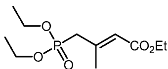
Compound 12
