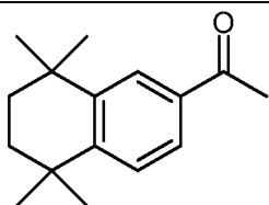
Compound 15
