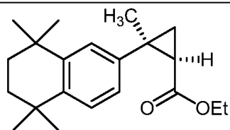
Compound 34
