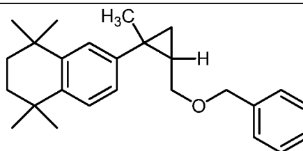
Compound 30
