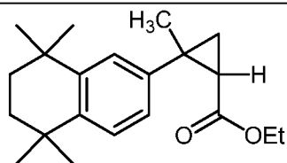
Compound 33
