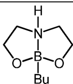
Compound 27
