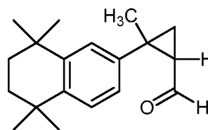
Compound 32
