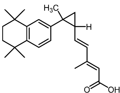
Compound 38,
