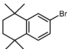
(Compound 3),
