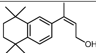
Compound 8
