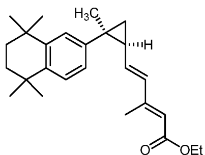
(Compound 13)
