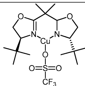
Compound 10
