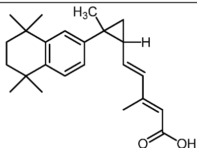
Compound 38
