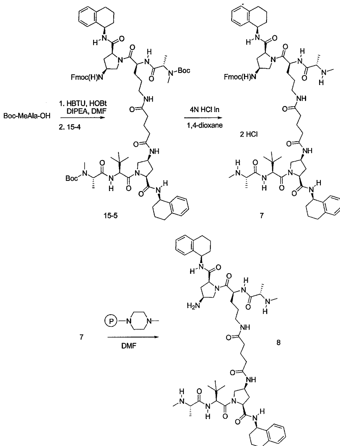
Scheme 15
