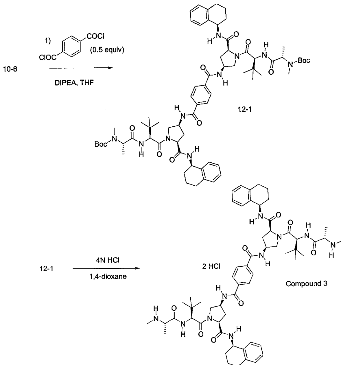
Scheme 12
