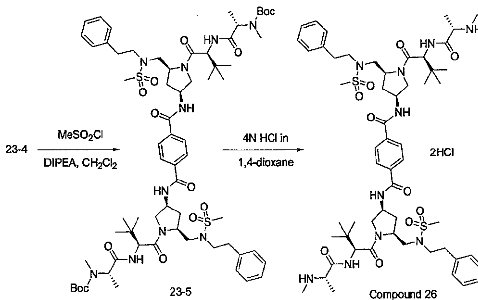
Scheme 23b
