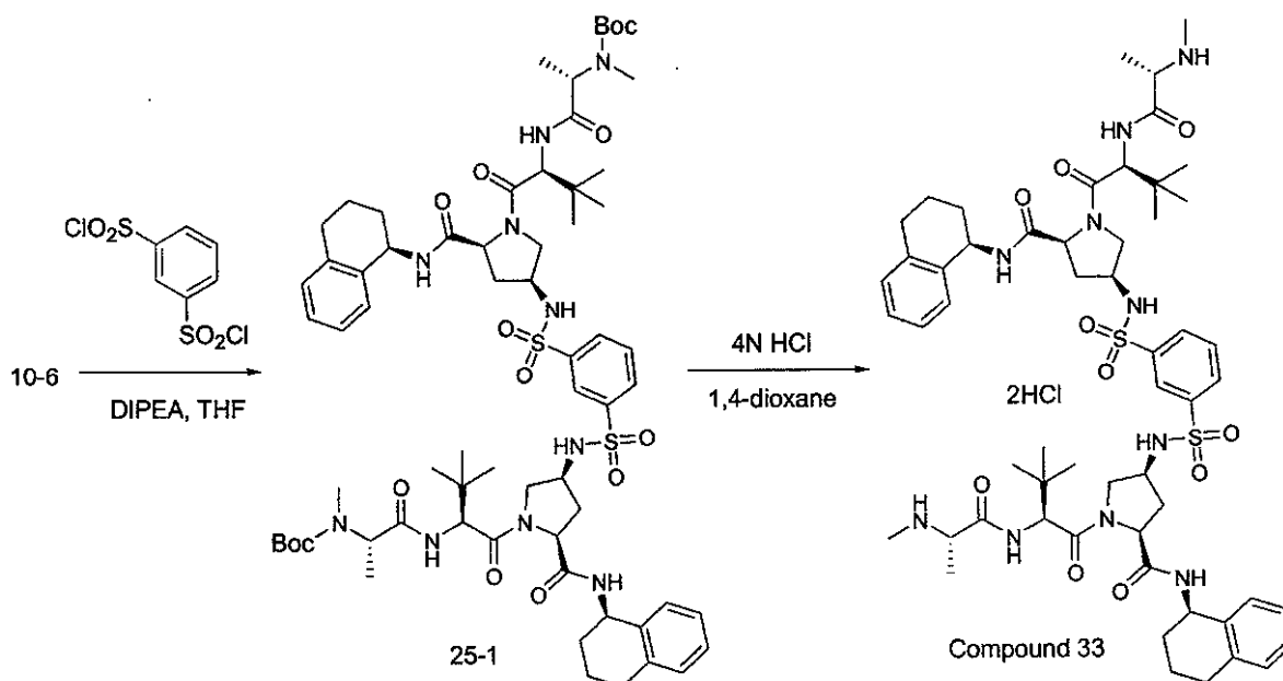
Scheme 25
