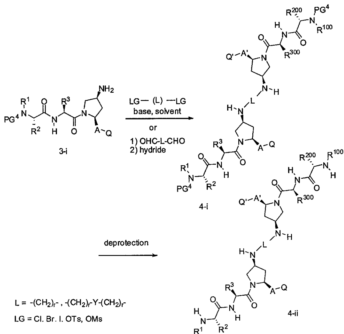
Scheme 4
