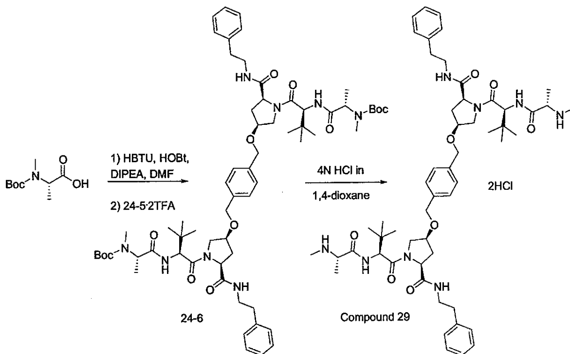
Scheme 24
