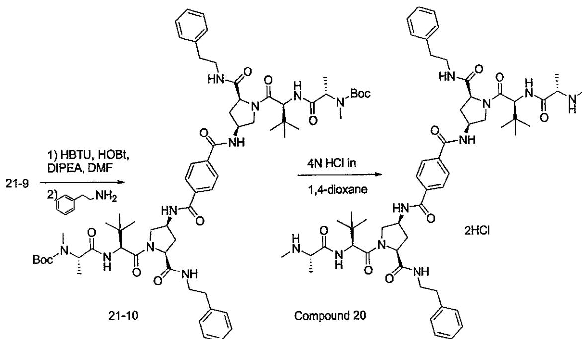
Scheme 21
