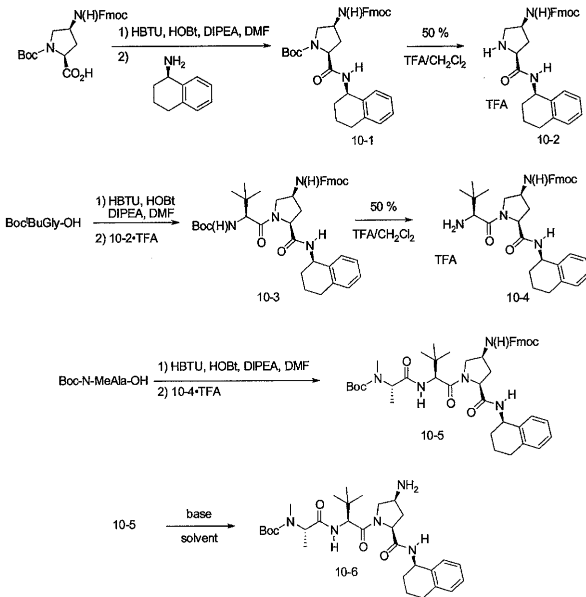
Scheme 10
