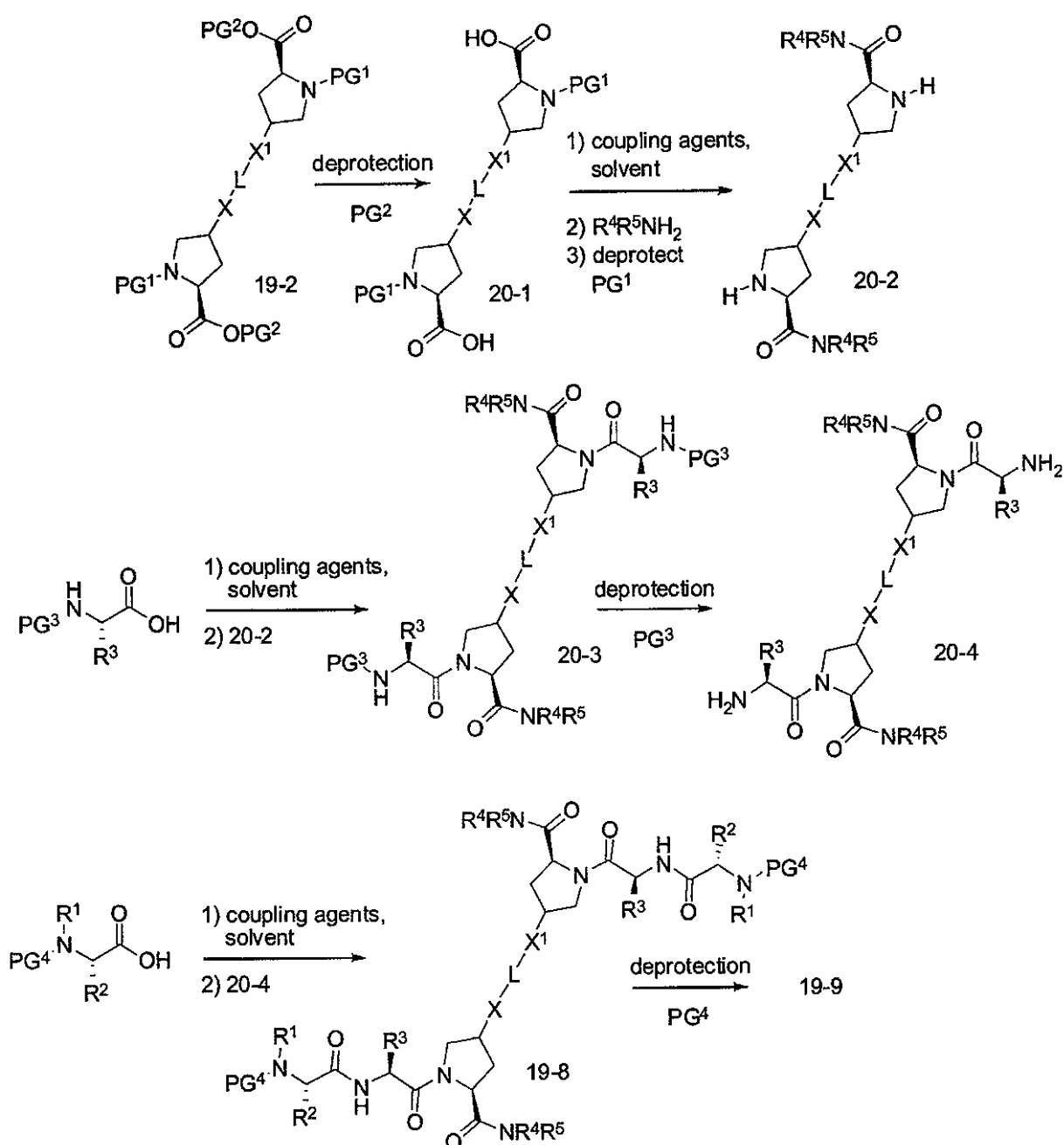
Scheme 20
