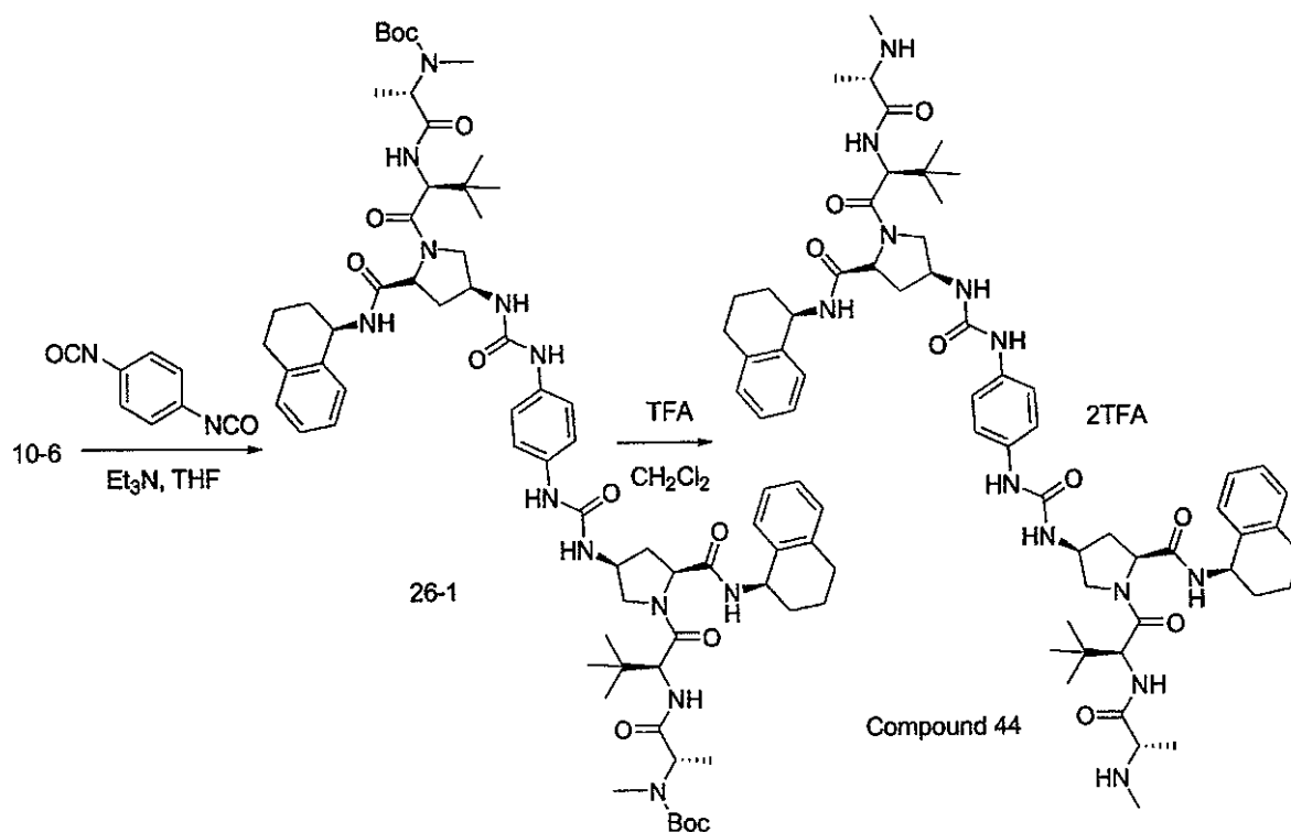
Scheme 26
