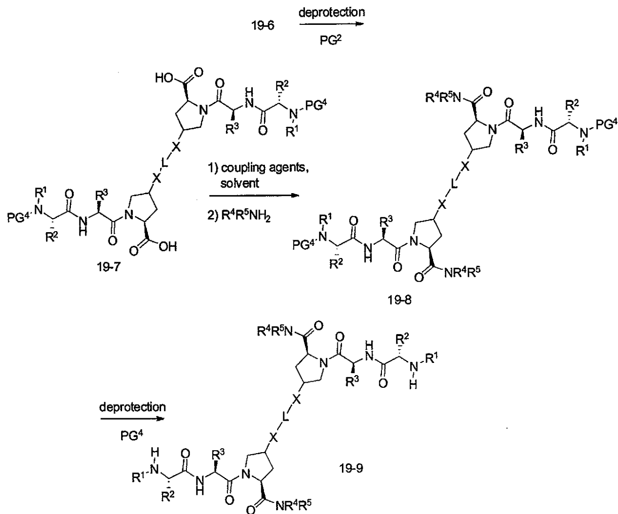
Scheme 19b
