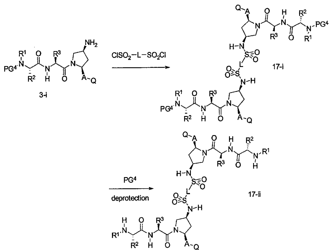
Scheme 17
