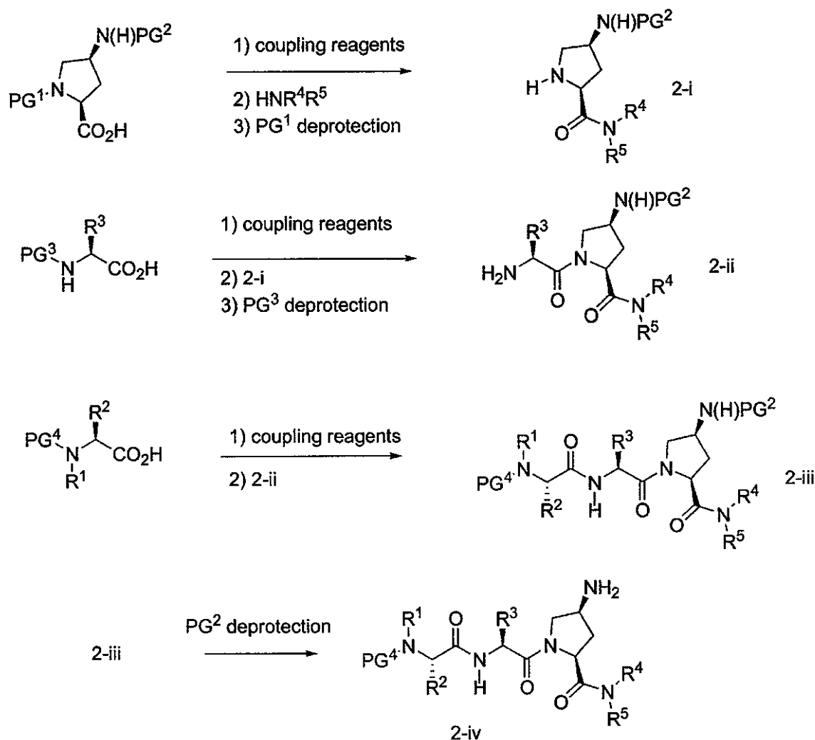
Scheme 2
