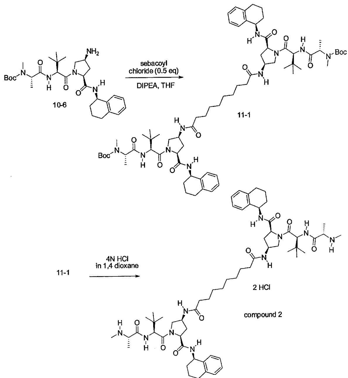
Scheme 11
