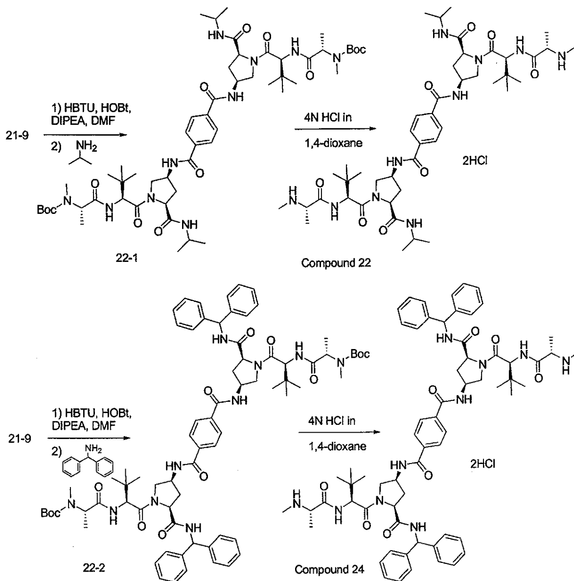
Scheme 22
