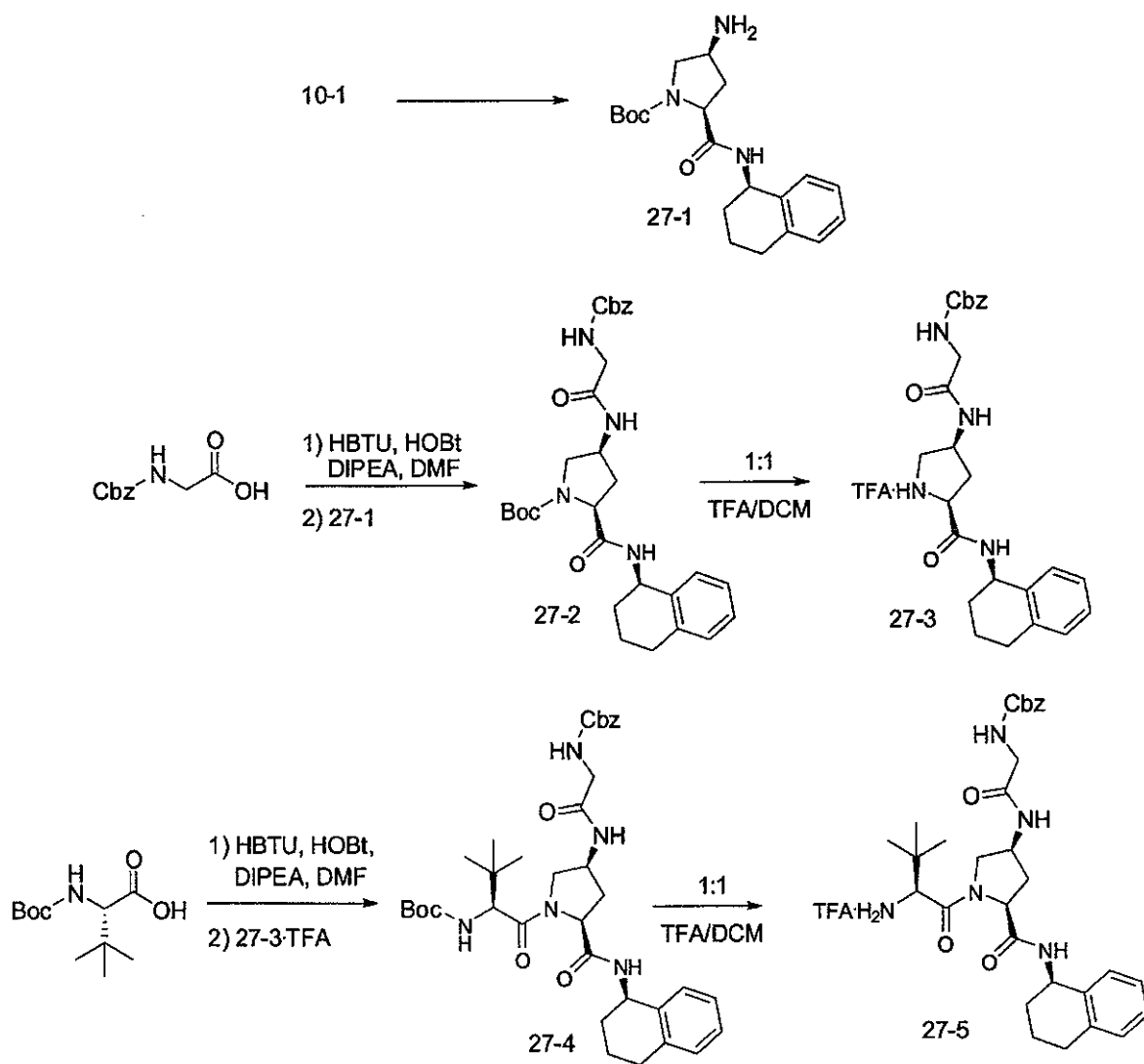
Scheme 27a
