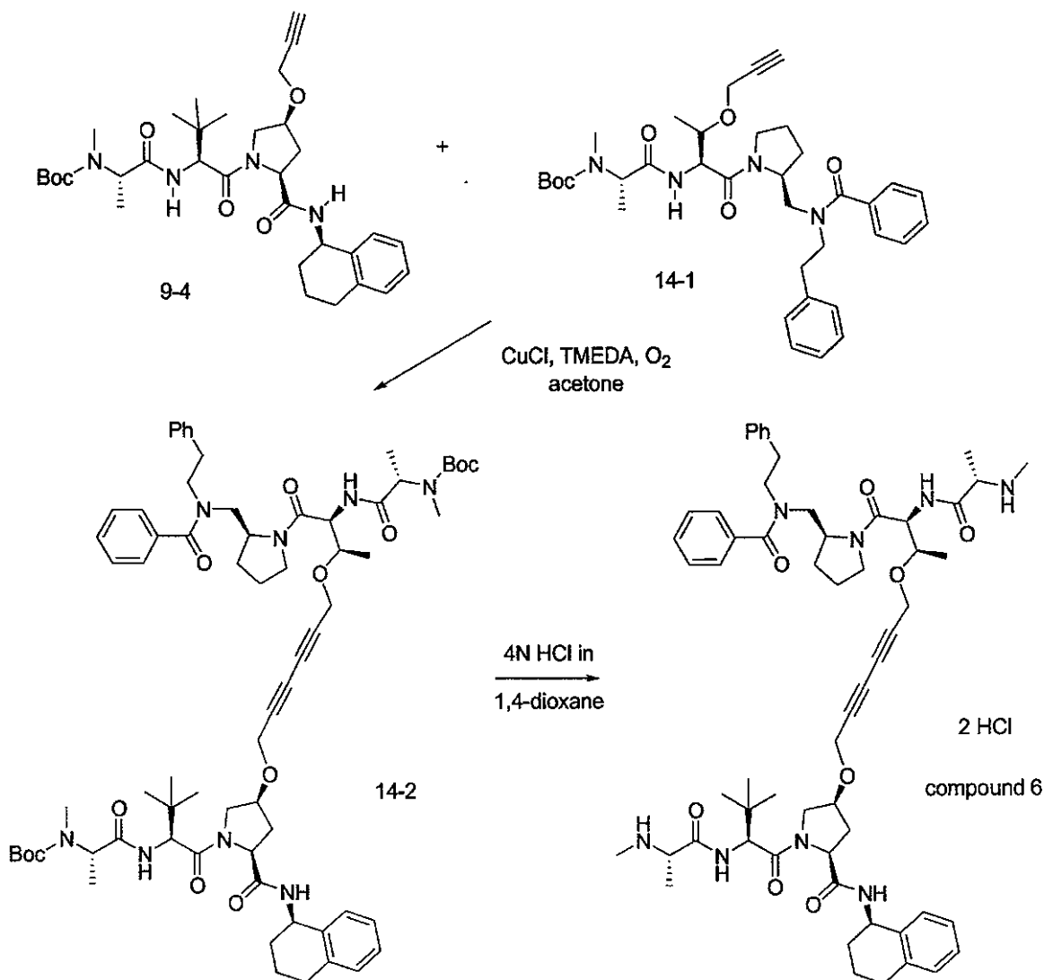
Scheme 14:
