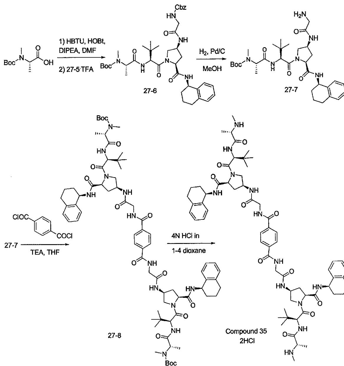
Scheme 27b
