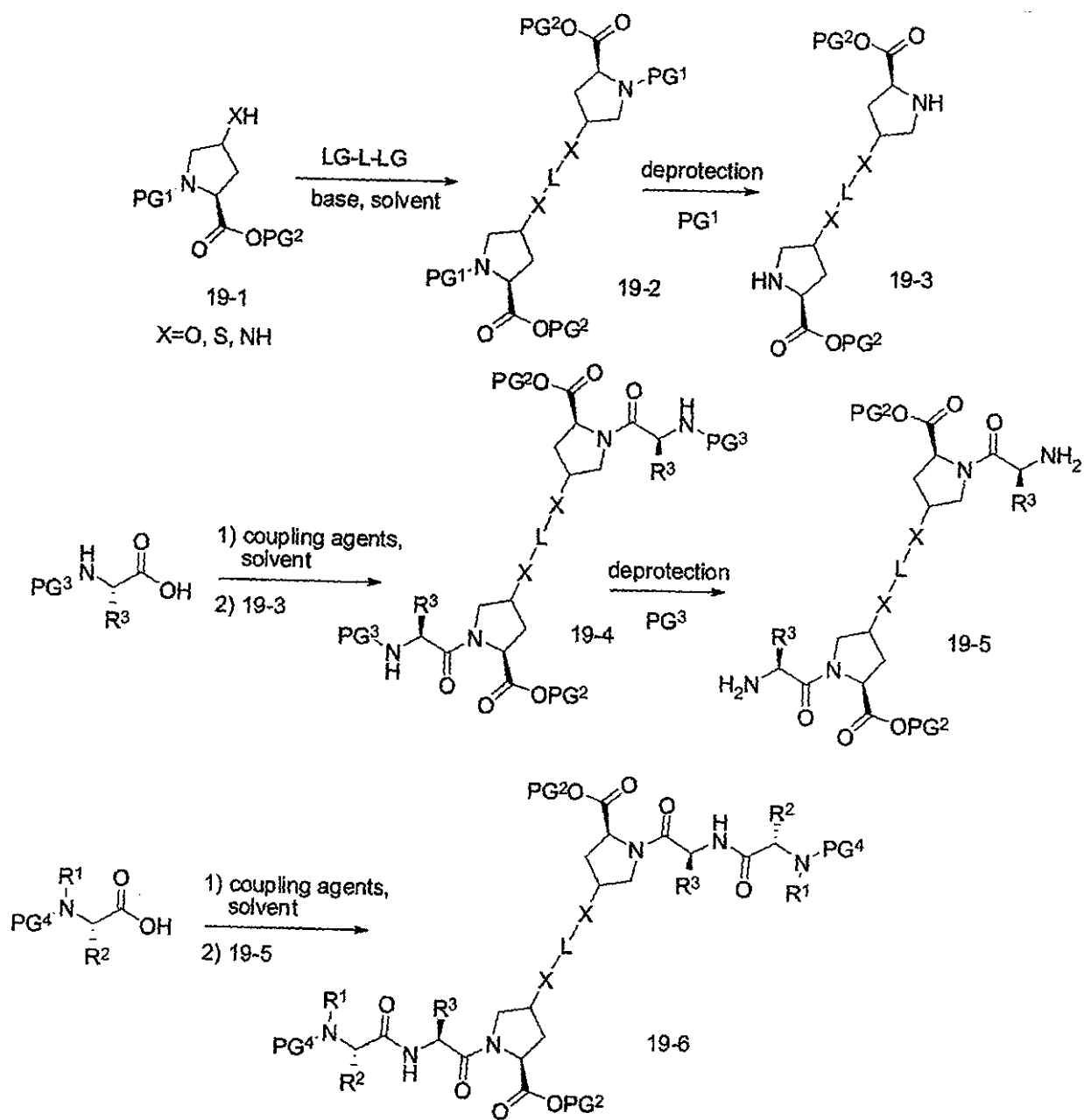
Scheme 19a
