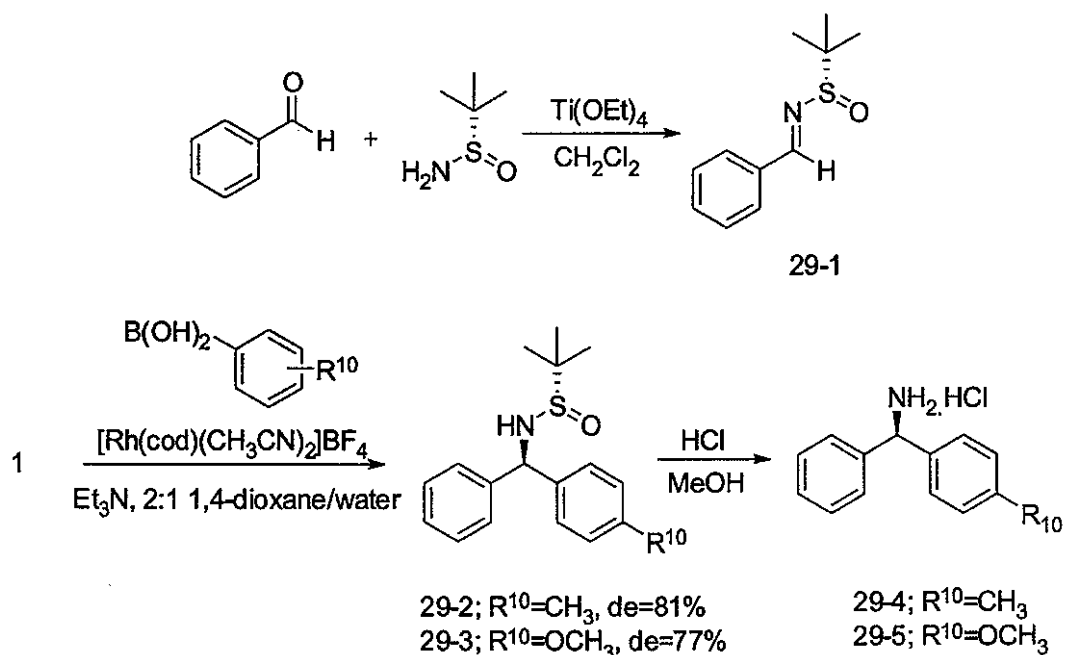
Scheme 29
