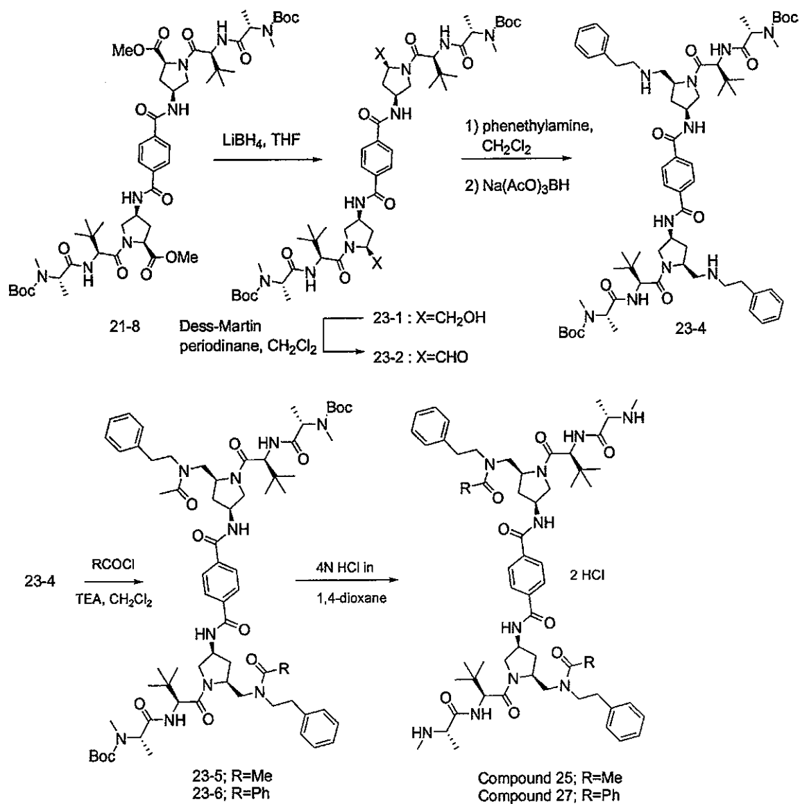
Scheme 23a
