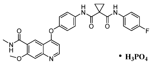
Compound 1 Phosphate Form A
