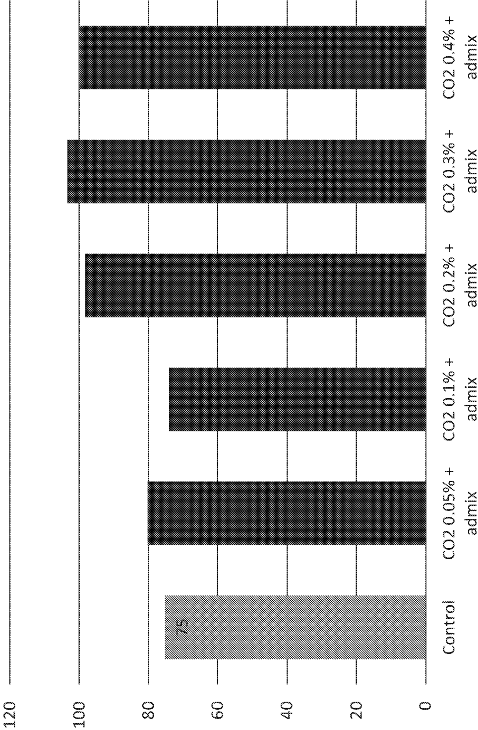
Figure 18 20 hr energy release (J/g cement)
