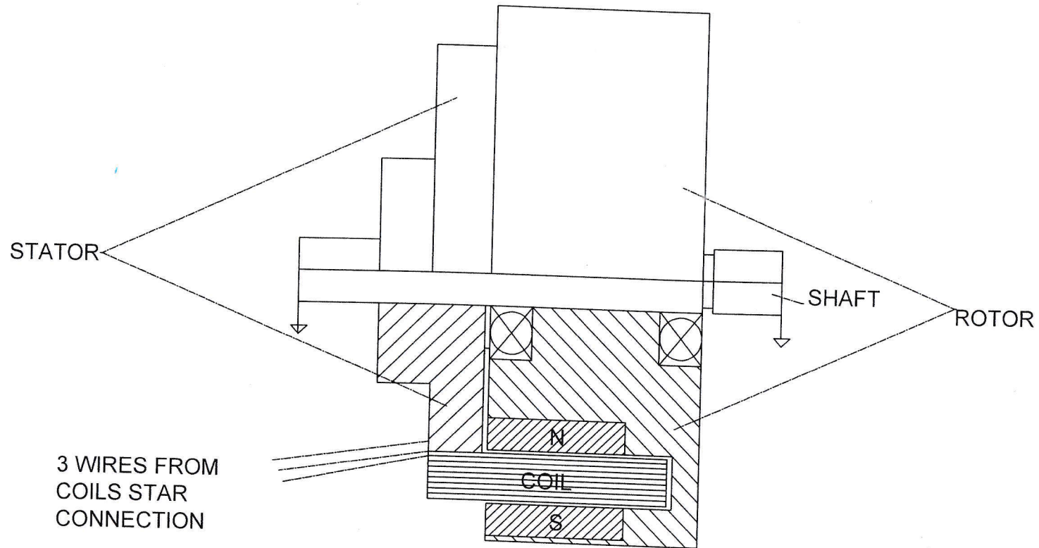
ASSEMBLY OF INTEGRATED LAYER ALTERNATOR / GENERATOR
