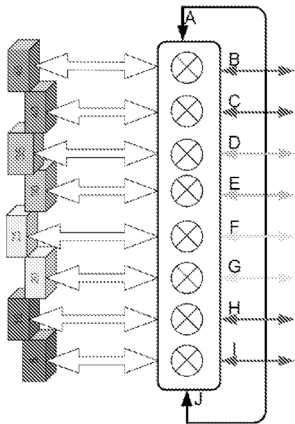
FIG 10B TemperatureGradient Heat Exchanger
