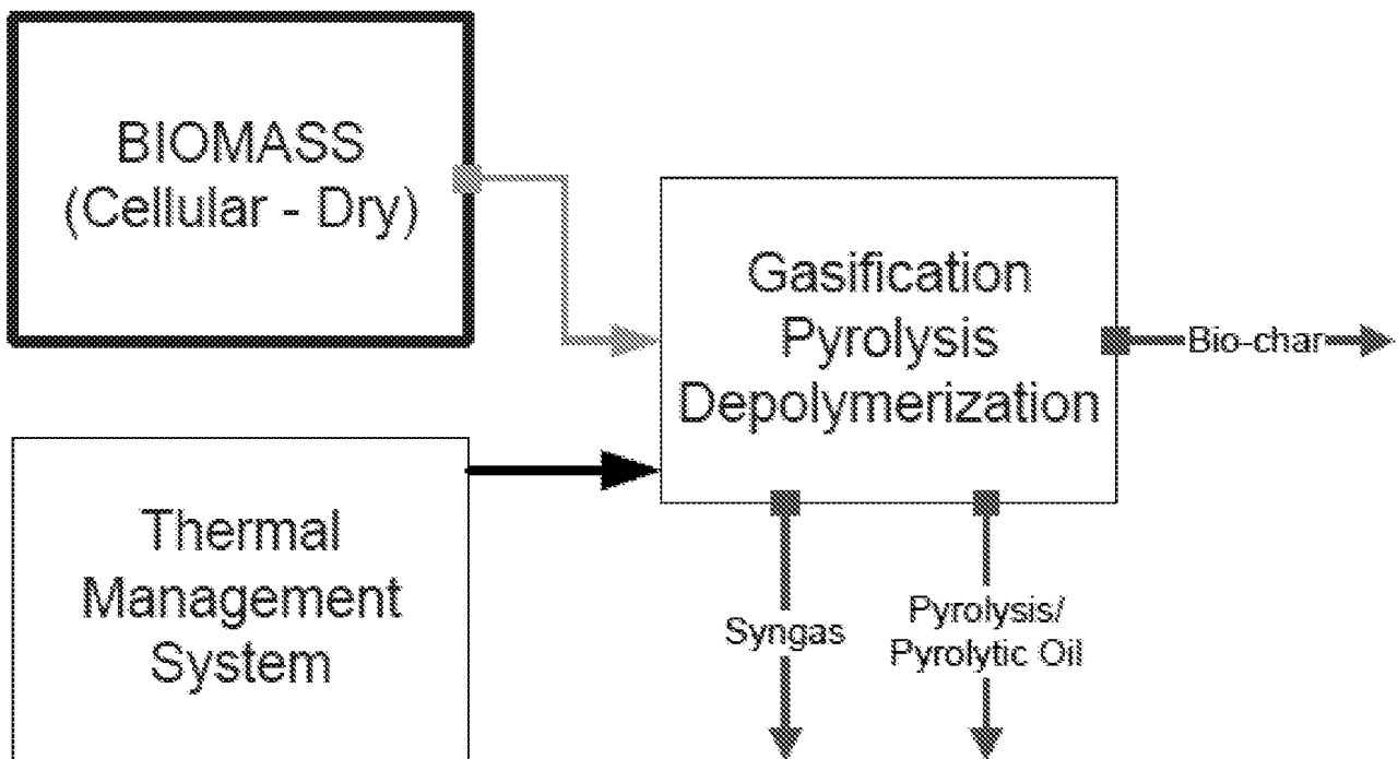
FIG 14 Thermochemical Processing
