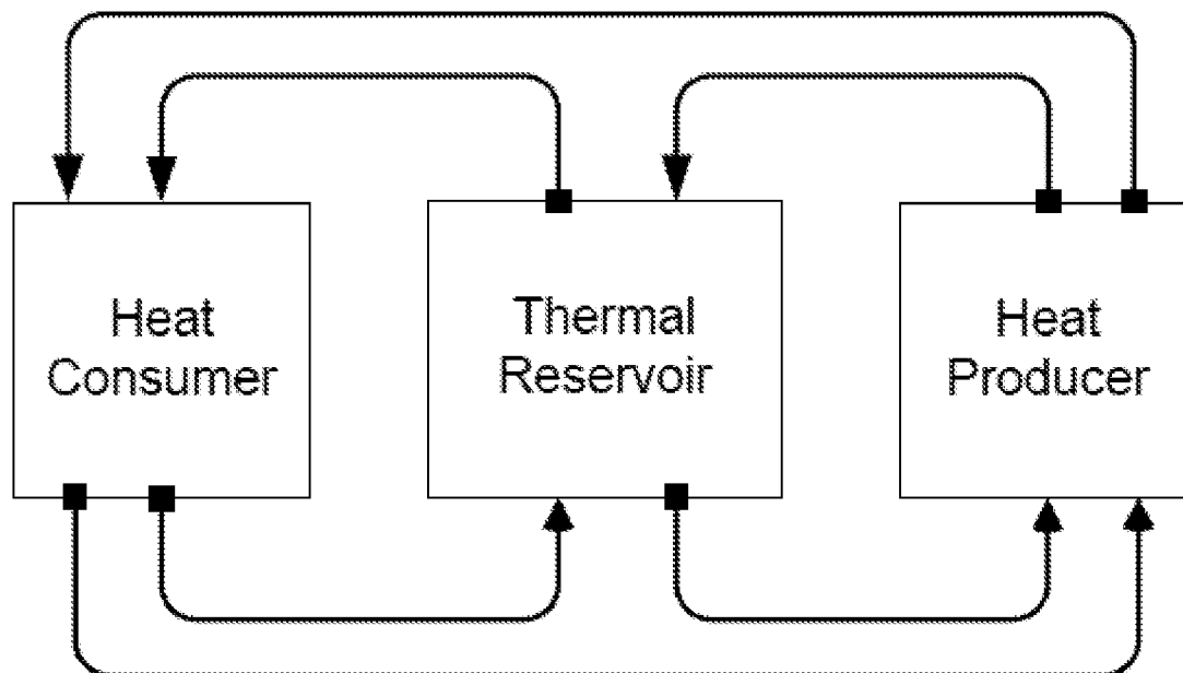
FIG 15 Consumer & Producer with Thermal Reservoir
