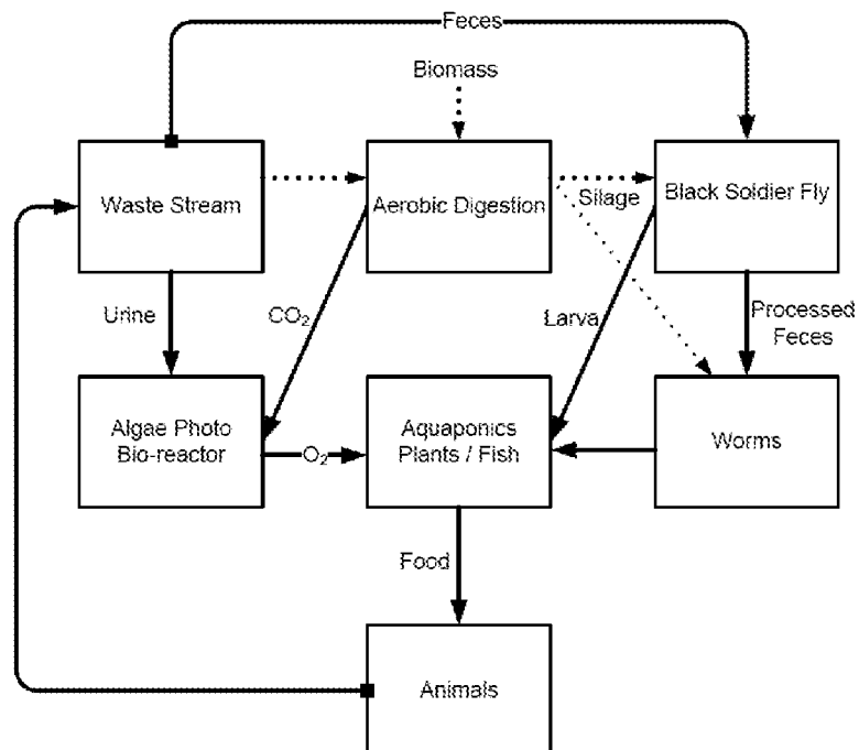
FIG 12 Waste Streams
