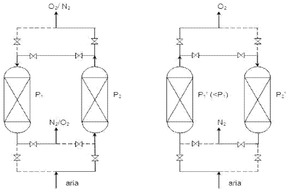
FIG 1 Pressure Swing Adsorption
