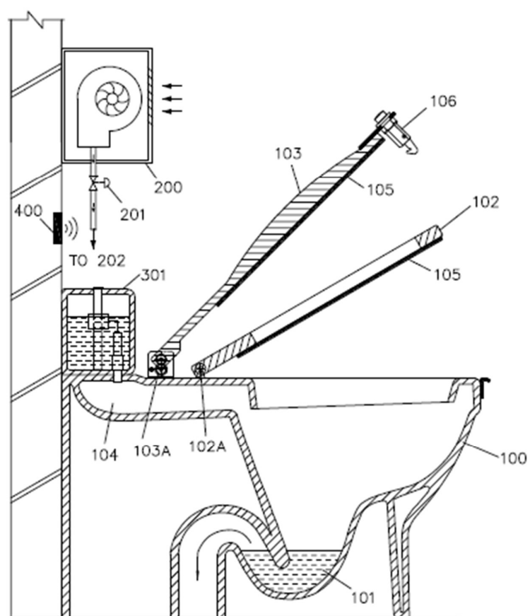
SECTION VIEW
