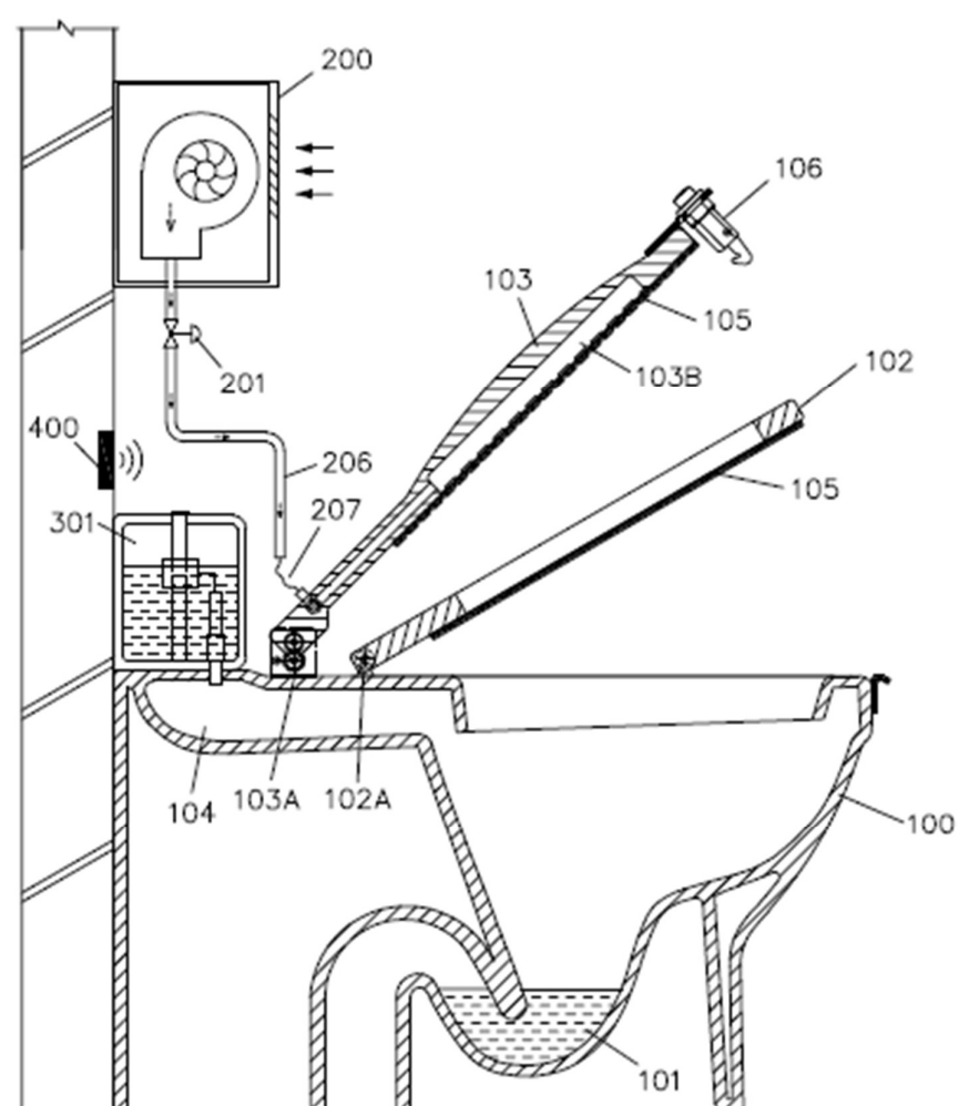
SECTION VIEW
