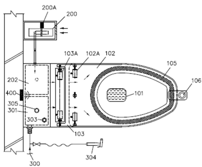
PLAN VIEW
