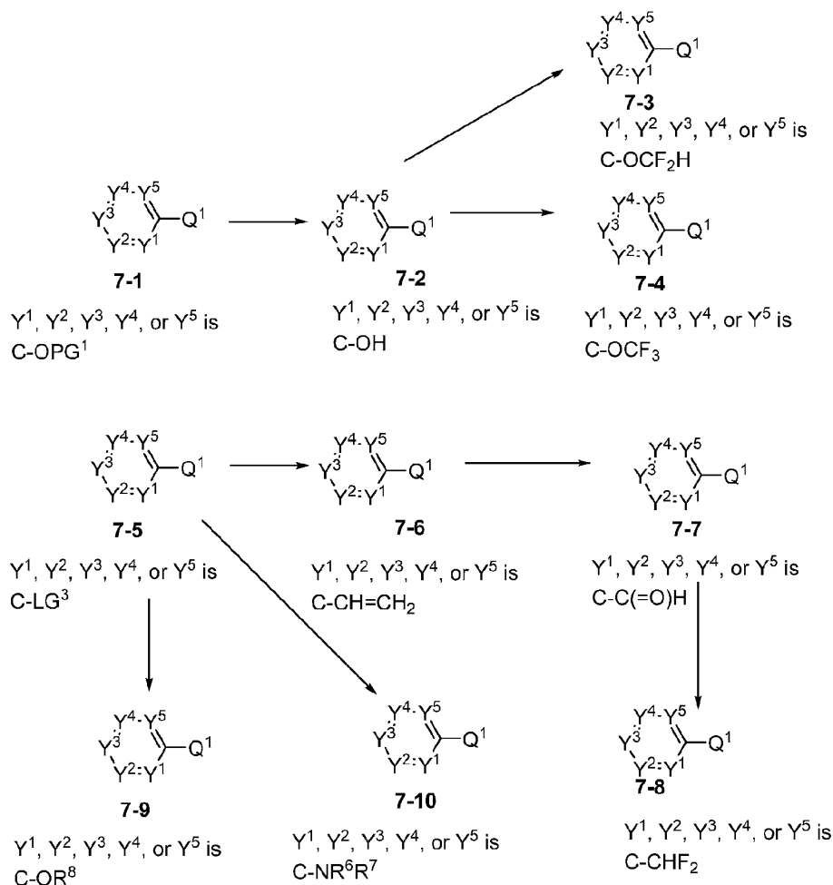
Scheme 7
