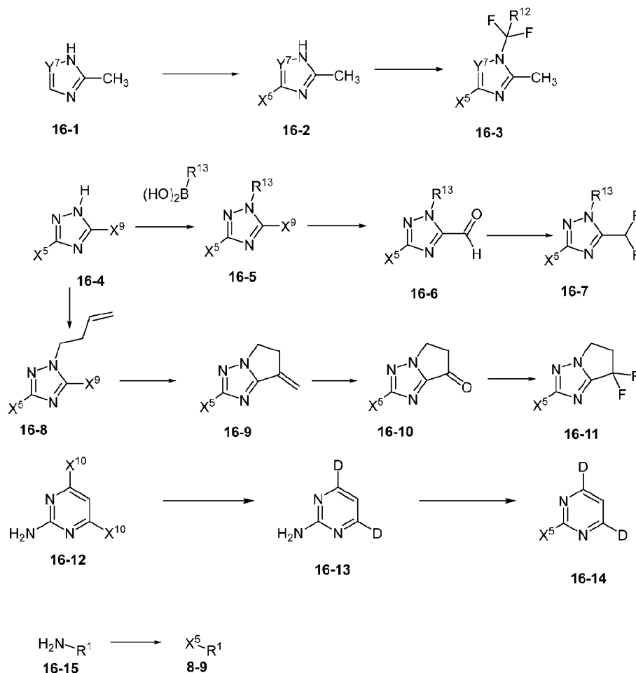
Scheme 16
