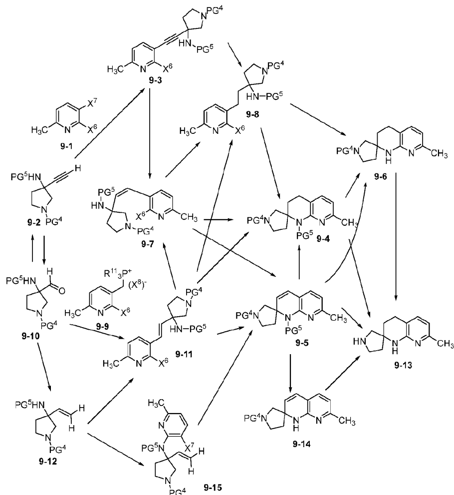
Scheme 9
