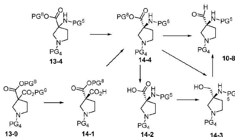
Scheme 14
