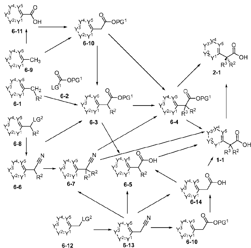
Scheme 6
