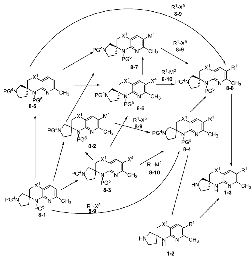
Scheme 8
