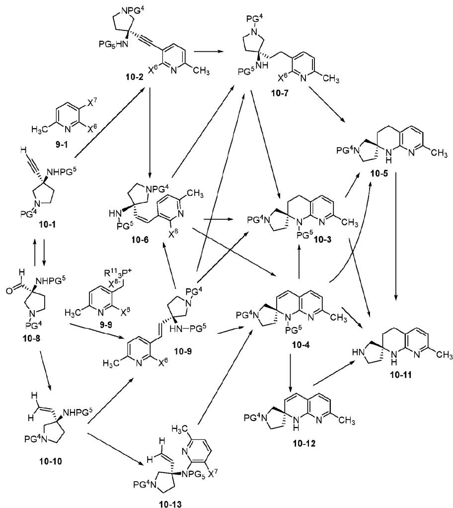
Scheme 10
