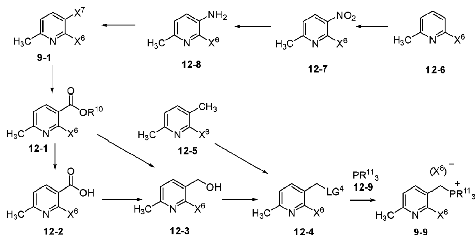
Scheme 12
