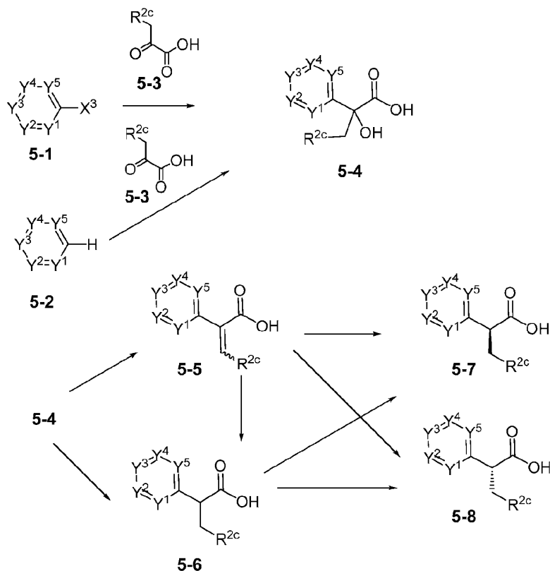
Scheme 5
