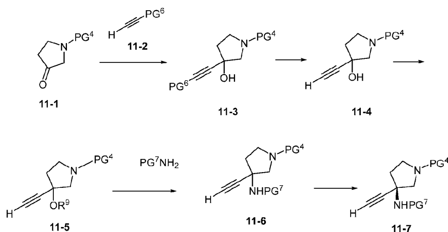
Scheme 11
