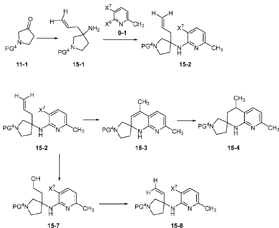
Scheme 15
