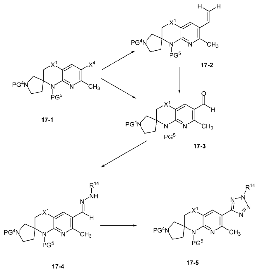
Scheme 17
