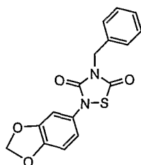
2-Benzo[1,3]dioxol-5-yl-4-benzyl-[1,2,4]thiadiazolidine-3,5-dione
