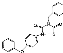
4-BENZYL-2-(4-PHENOXY-PHENYL)-[1,2,4]THIADIAZOLIDINE-3,5-DIONE
