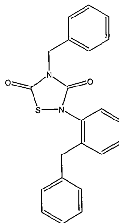
4-Benzyl-2-(2-benzyl-phenyl)-[1,2,4]thiadiazolidine-3,5-dione
