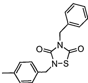
4-Benzyl-2-(4-methyl-benzyl)-[1,2,4]thiadiazolidine-3,5-dione
