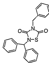
4-Benzyl-2-diphenylmethyl-1,2,4-thiadiazolidine-3,5-dione
