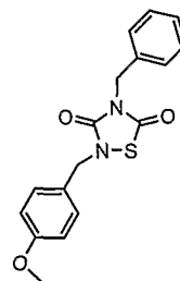
4-Benzyl-2-(4-methoxy-benzyl)-[1,2,4]thiadiazolidine-3,5-dione
