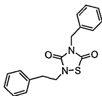
4-Benzyl-2-phenethyl-[1,2,4]thiadiazolidine-3,5-dione
