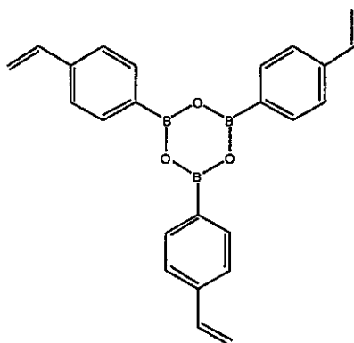
Structure III
