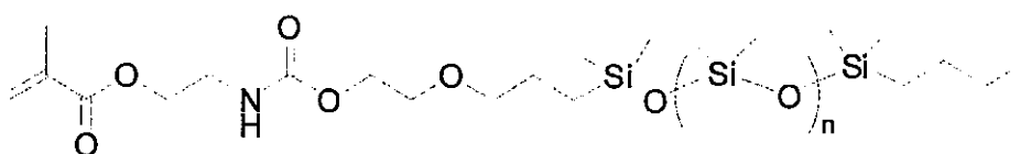
Silicone B
