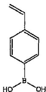
Structure IV
