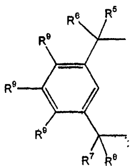
(XXIII) and
