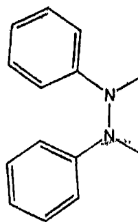
(XXIII) and
