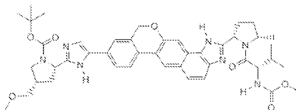
Compound II
