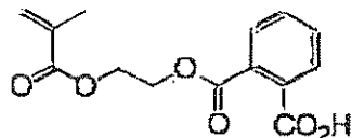
Monomer d
