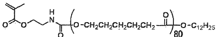
Macromonomer (2-5)
