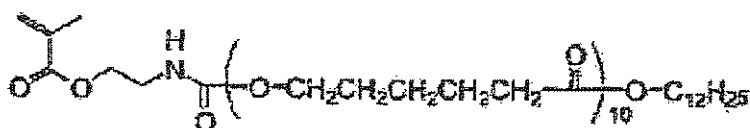
Macromonomer (2-1)
