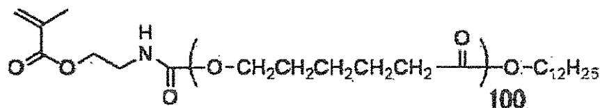
Macromonomer (2-7)
