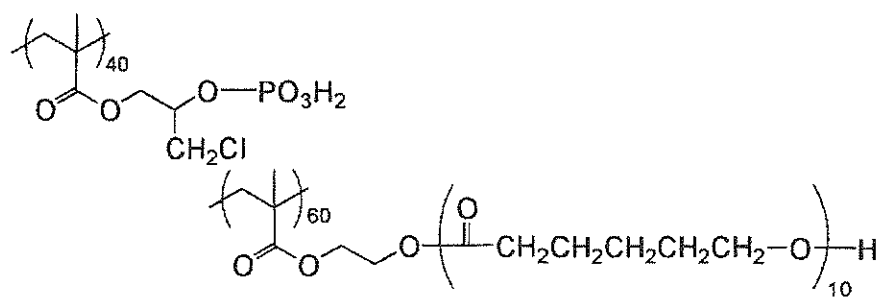
(B-1-4) Mw 28,000
