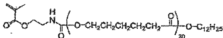
Macromonomer (2-2)
