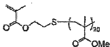
Macromonomer (2-3)
