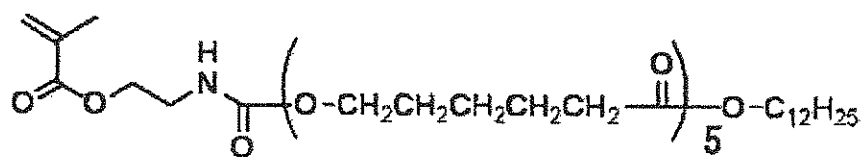
Macromonomer (2-4)
