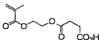
Monomer f
