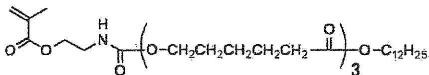
Macromonomer (2-6)
