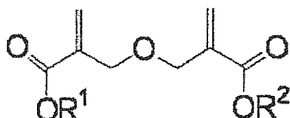
Formula (ED)
