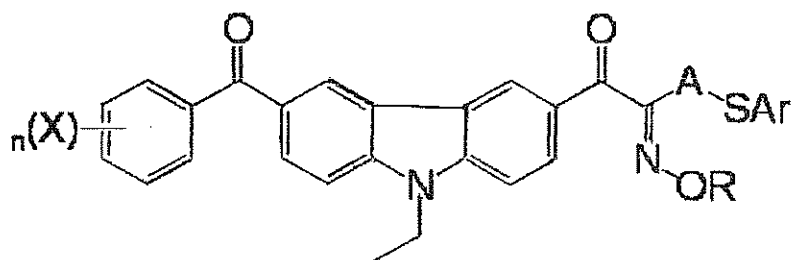
Formula (a)
