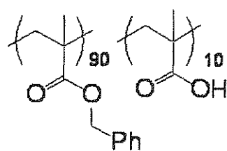
Resin (D-2)
