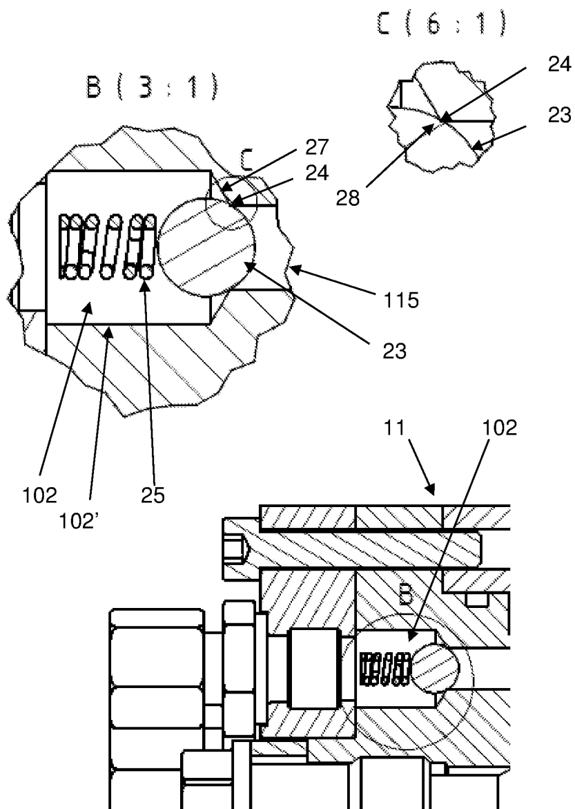
FIG. 4 (prior art)
