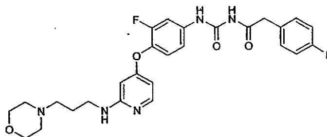
1-(3-Fluoro-4-(2-(3-morpholinopropylamino)pyridin-4-yloxy)phenyl)-3-(2-(4-fluorophenyl)acetyl)urea, hydrochloride salt
