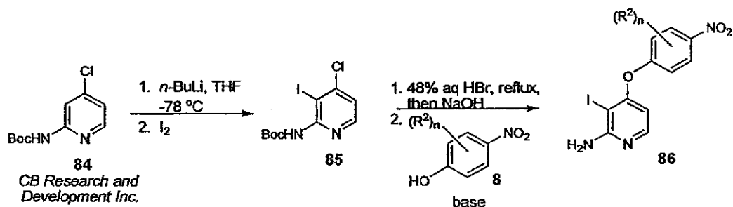
SCHEME 16
