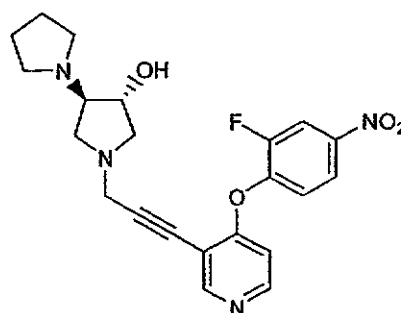
A) (3R,4R)-1-(3-(4-(2-Fluoro-4-nitrophenoxy)pyridin-3-yl)prop-2-yn-1-yl)-4-(pyrrolidin-1-yl)pyrrolidin-3-ol
