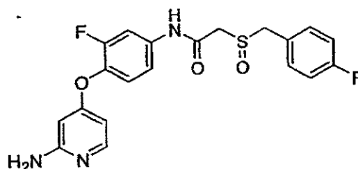
10 2-(4-Fluorobenzylsulfinyl)- N -(4-(2-aminopyridin-4-yloxy)-3-fluorophenyl)acetamide, hydrochloride salt
