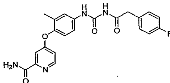
1-(4-(2-Carbamoylpyridin-4-yloxy)-3-methylphenyl)-3-(2-(4-fluorophenyl)acetyl)urea
