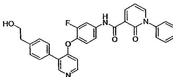
N -(3-Fluoro-4-(3-(4-(2-hydroxyethyl)phenyl)pyridin-4-yloxy)phenyl)-2-oxo-1-phenyl-1,2-dihydropyridine-3-carboxamide
