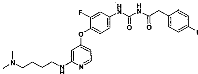
1-(4-(2-(4-(Dimethylamino)butylamino)pyridin-4-yloxy)-3-fluorophenyl)-3-(2-(4-fluorophenyl)acetyl)urea, hydrochloride salt
