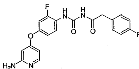
1-(4-(2-Aminopyridin-4-yloxy)-2-fluorophenyl)-3-(2-(4-fluorophenyl)acetyl)urea, trifluoroacetic acid salt
