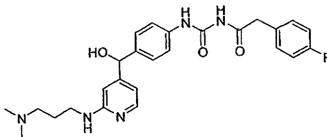
1-(4-((2-(3-(Dimethylamino)propylamino)pyridin-4-yl)(hydroxy)methyl)phenyl)- 3-(2-(4-fluorophenyl)acetyl)urea
