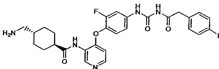
1-(4-(3-((1R,4R)-4-(Aminomethyl)cyclohexanecarboxamido)pyridin-4-yloxy)-3-fluorophenyl)-3-(2-(4-fluorophenyl)acetyl)urea
