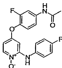
20 A) N-(3-Fluoro-4-(2-(4-fluorophenylamino)pyridin-4-yloxy-1-oxide)phenyl)acetamide
