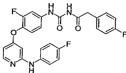
15 1-(3-Fluoro-4-(2-(4-fluorophenylamino)pyridin-4-yloxy)phenyl)-3-(2-(4-fluorophenyl)acetyl)urea
