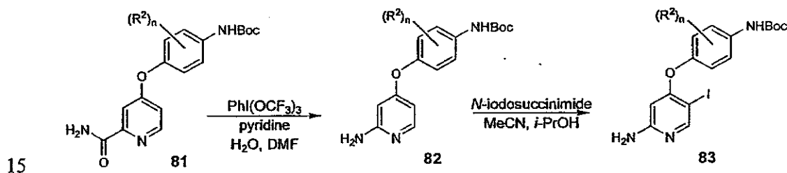
SCHEME 15
