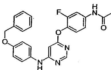
A) N -(4-(6-(4-(Benzyloxy)phenylamino)pyrimidin-4-yloxy)-3-fluorophenyl)acetamide
