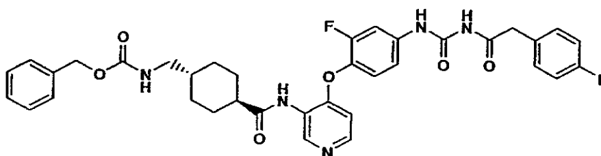
1-(4-(3-((1R,4R)-4-(Aminomethyl)cyclohexanecarboxamido)pyridin-4-yloxy)-3-fluorophenyl)-3-(2-(4-fluorophenyl)acetyl)urea
