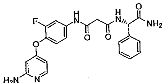
(S)-N 1 -(2-Amino-2-oxo-1-phenylethyl)-N 3 -(4-(2-aminopyridin-4-yloxy)-3-fluorophenyl)malonamide, hydrochloride salt
