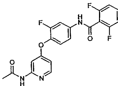
N -(4-(2-Acetamidopyridin-4-yloxy)-3-fluorophenyl)-2,6-difluorobenzamide, hydrochloride salt
