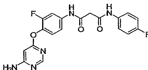
N 1 -(4-(6-Aminopyrimidin-4-yloxy)-3-fluorophenyl)- N 3 -(4-fluorophenyl)malonamide
