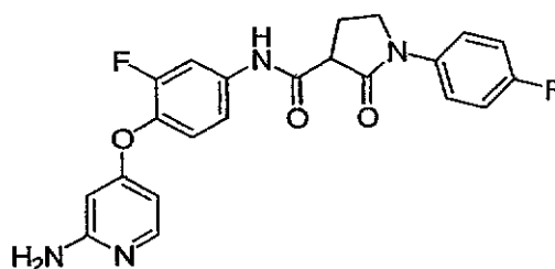
N -(4-(2-Aminopyridin-4-yloxy)-3-fluorophenyl)-1-(4-fluorophenyl)-2-oxopyrrolidine-3-carboxamide
