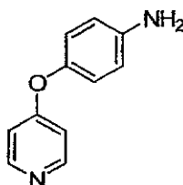
N -(4-Fluorophenyl)- N -(4-(pyridin-4-yloxy)phenyl)malonamide
