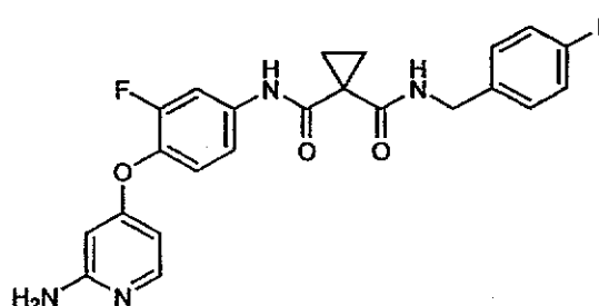
N-(4-Fluorobenzyl)-N-(4-(2-aminopyridin-4-yloxy)-3-fluorophenyl)cyclopropane-1,1-dicarboxamide
