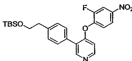
N -(3-Fluoro-4-(3-(4-(2-hydroxyethyl)phenyl)pyridin-4-yloxy)phenyl)-2-oxo-1-phenyl-1,2-dihydropyridine-3-carboxamide
