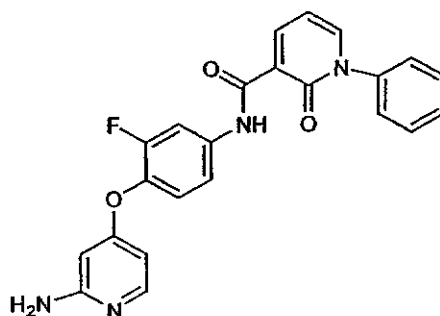
N -(4-(2-Aminopyridin-4-yloxy)-3-fluorophenyl)-2-oxo-1-phenyl-1,2-dihydropyridine-3-carboxamide, trifluoroacetic acid salt
