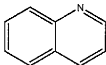
quinoline
