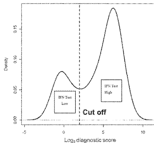
Distribution of IFN transcript scores
