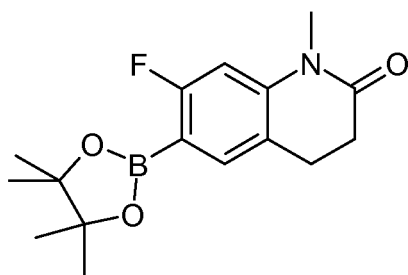
[B] 7-Fluoro-1-methyl-6-(4,4,5,5-tetramethyl-[1,3,2]dioxaborolan-2-yl)-3,4-dihydro-1H-quinolin-2-one
