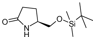
[A] (S)-5-( tert -Butyl-dimethyl-silanyloxymethyl)-pyrrolidin-2-one
