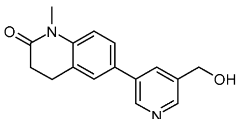
[A] 6-(5-Hydroxymethyl-pyridin-3-yl)-1-methyl-3,4-dihydro-1H-quinolin-2-one
