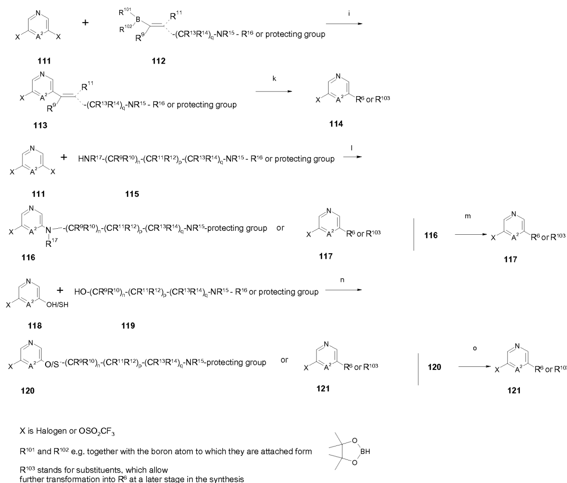
Scheme 2b
