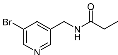
[A] N -(5-Bromo-pyridin-3-ylmethyl)-propionamide
