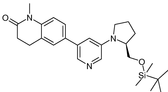
[A] (S)-2-( tert -Butyl-dimethyl-silanyloxymethyl)-pyrrolidine
