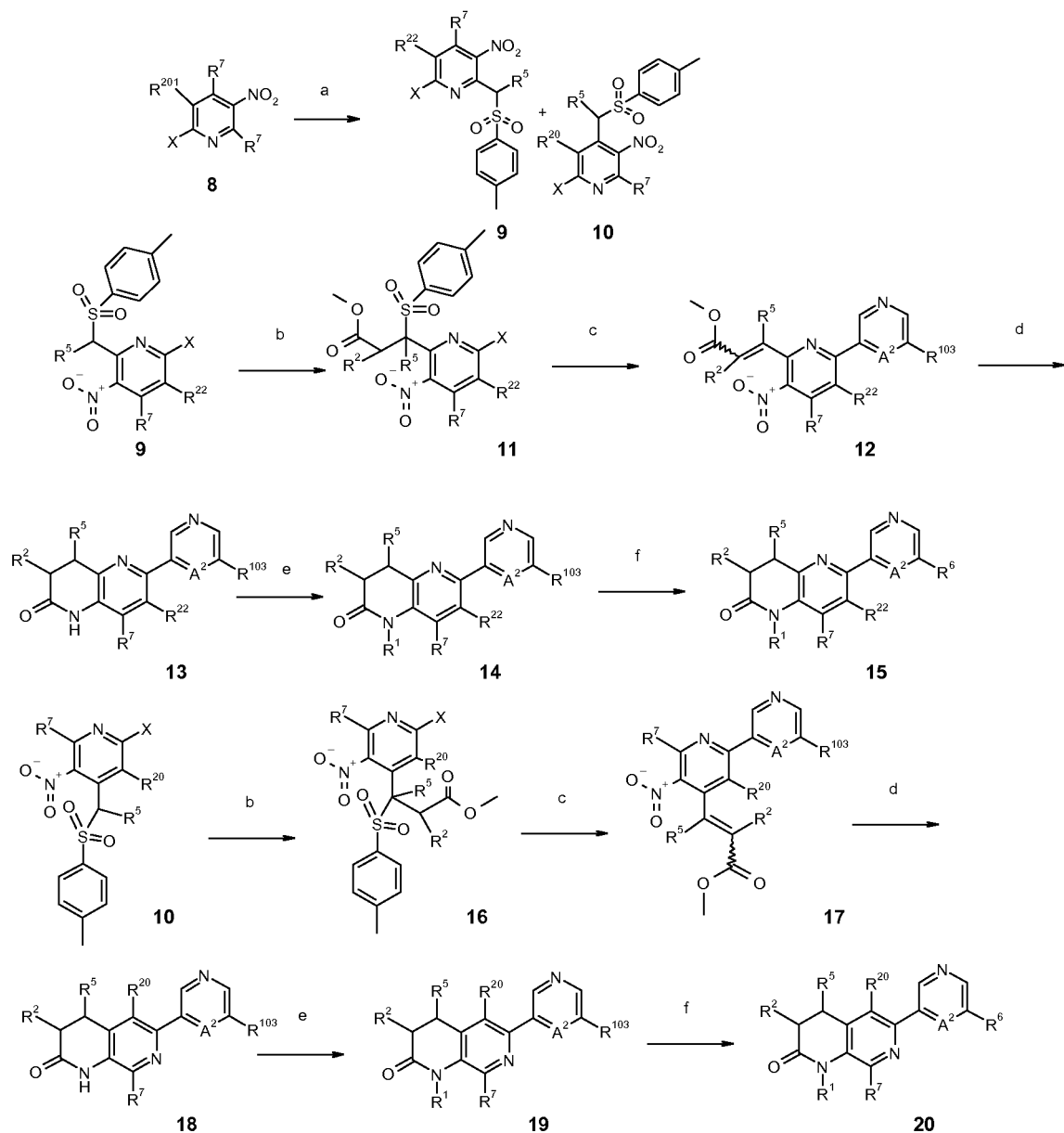
Scheme 1b
