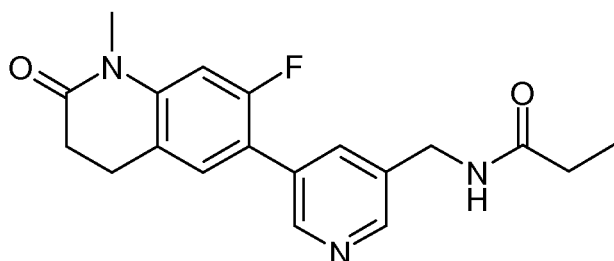
[B] N -[5-(7-Fluoro-1-methyl-2-oxo-1,2,3,4-tetrahydro-quinolin-6-yl)-pyridin-3-ylmethyl]- propionamide
