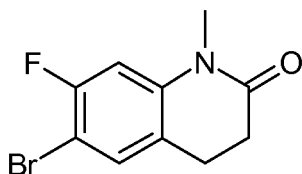
[A] 6-Bromo-7-fluoro-1-methyl-3,4-dihydro-1H-quinolin-2-one
