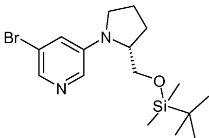
[B] 3-Bromo-5-[(R)-2-( tert -butyl-dimethyl-silanyloxymethyl)-pyrrolidin-1-yl]-pyridine
