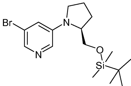
10 [B] 3-Bromo-5-[(S)-2-( tert -butyl-dimethyl-silanyloxymethyl)-pyrrolidin-1-yl]-pyridine
